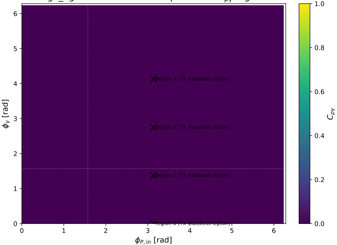
high_Egamma Tx massless lepton: max C_{p\gamma} regions
