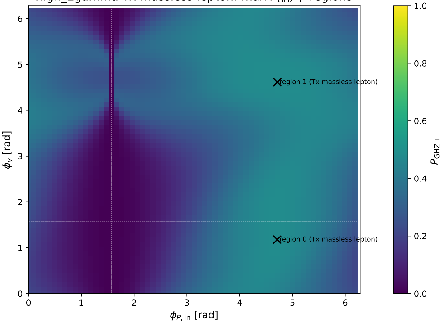
high_Egamma Tx massless lepton: max P_{\text{GHZ}+} regions
