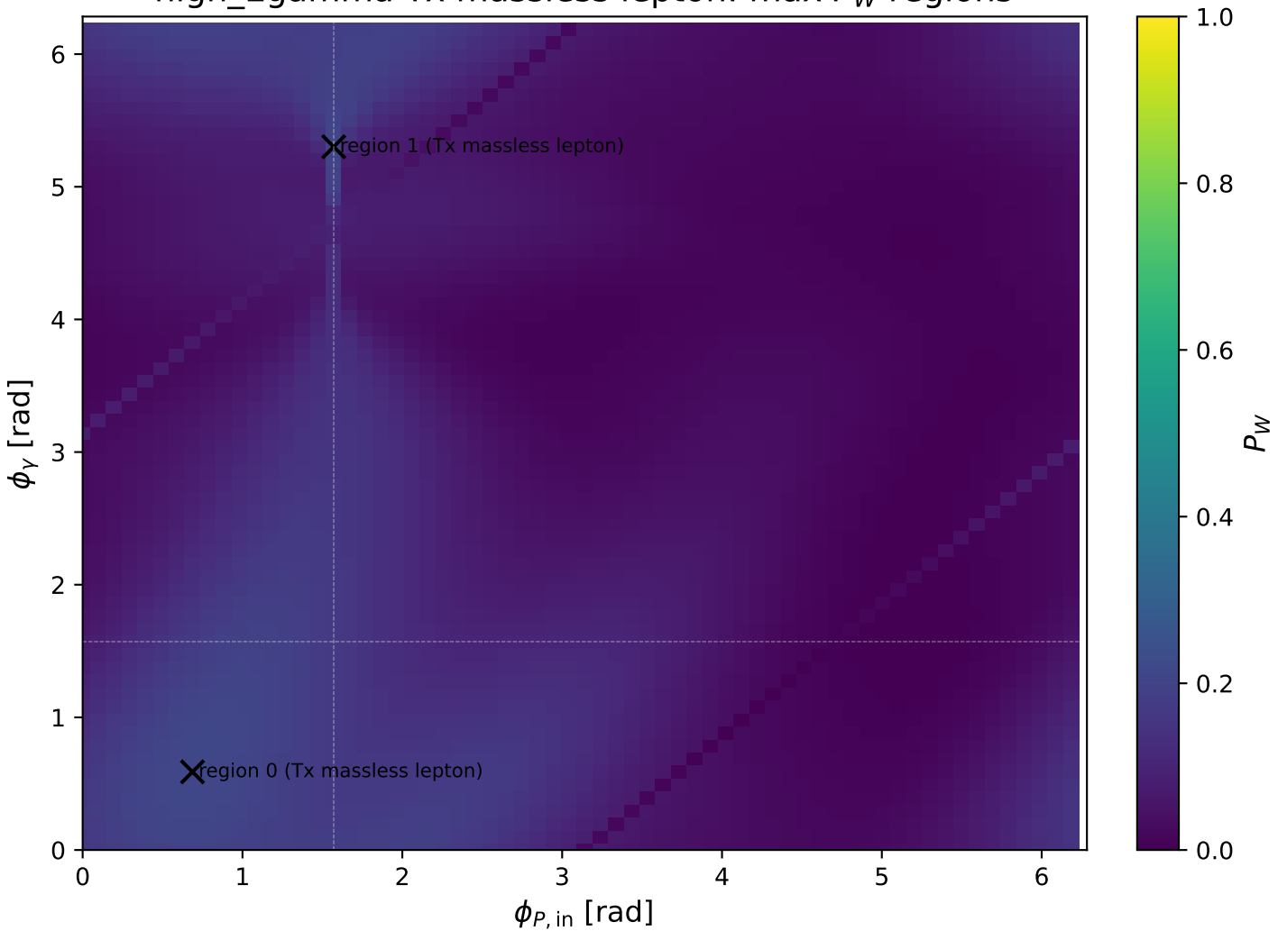
high_Egamma Tx massless lepton: max P_W regions
