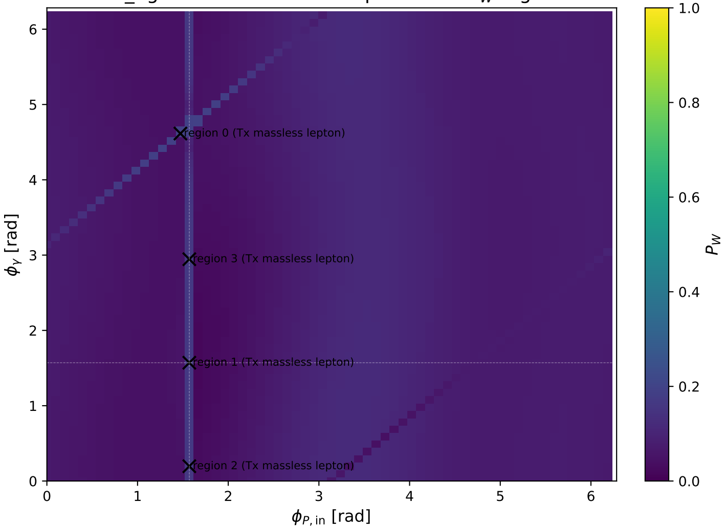
low_Egamma Tx massless lepton: max P_W regions
