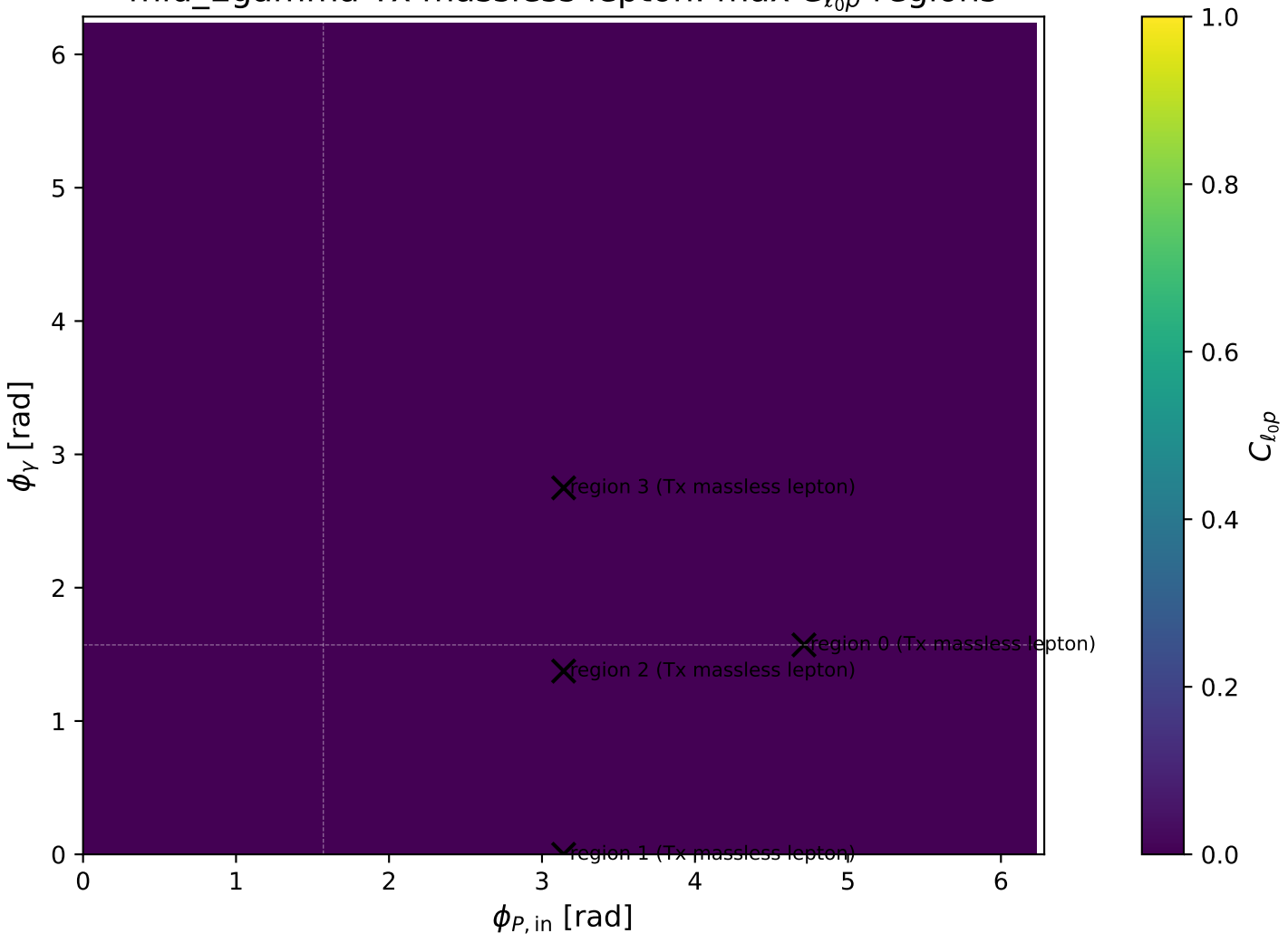
mid_Egamma Tx massless lepton: max C_{\ell_0 p} regions
