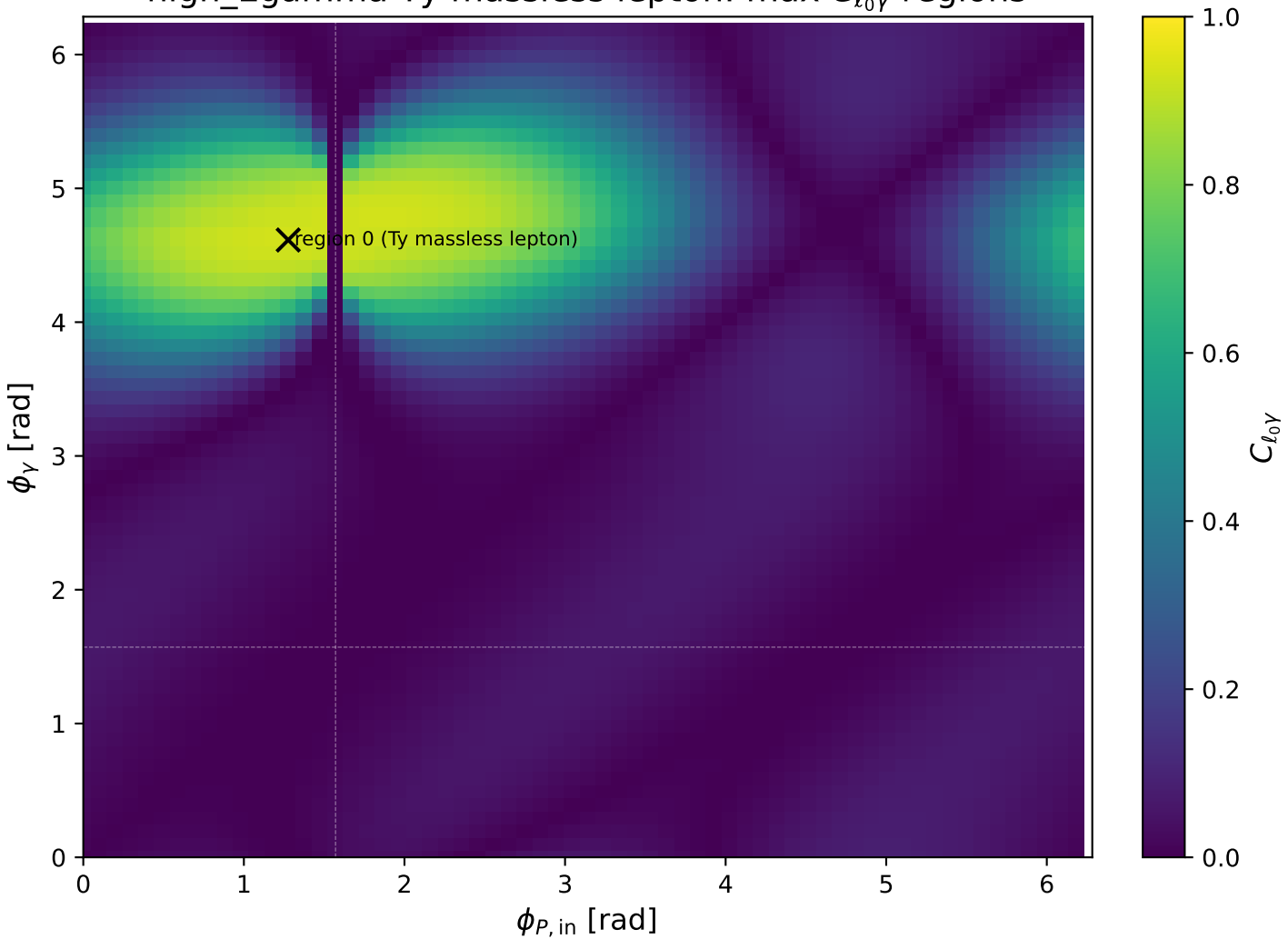
high_Egamma Ty massless lepton: max C_{\ell_0\gamma} regions
