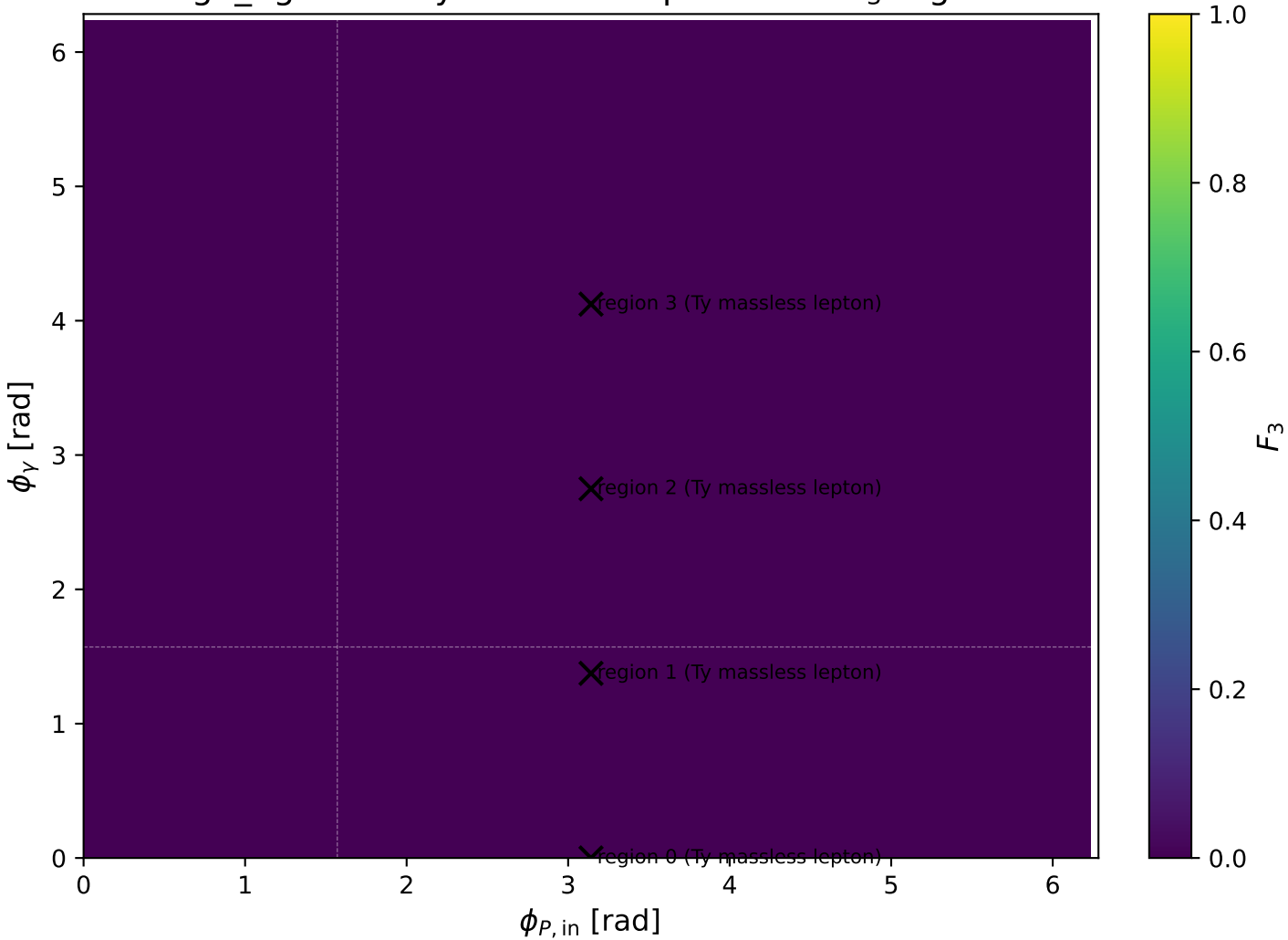
high_Egamma Ty massless lepton: max F_3 regions
