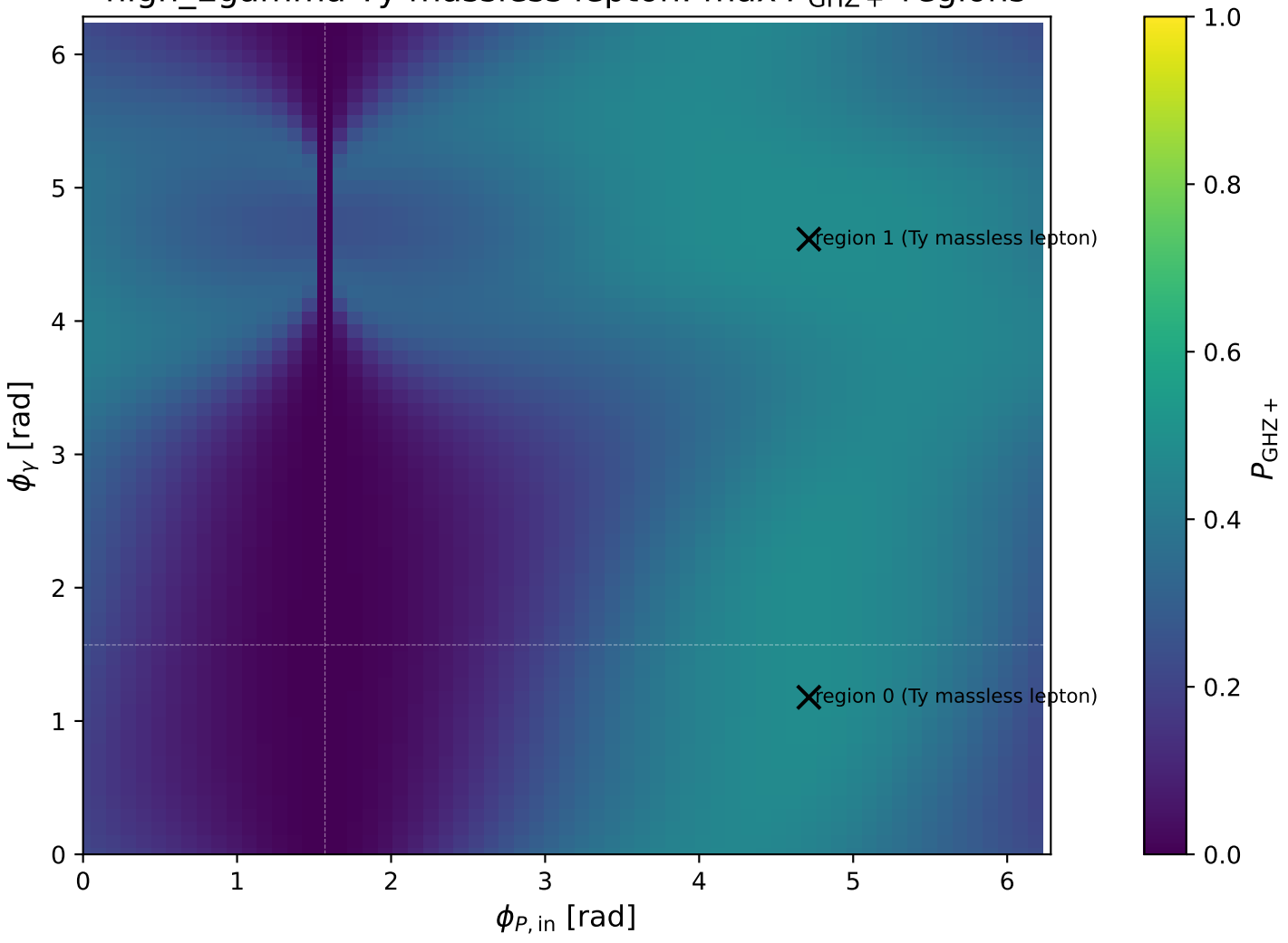
high_Egamma Ty massless lepton: max P_{\text{GHZ}+} regions
