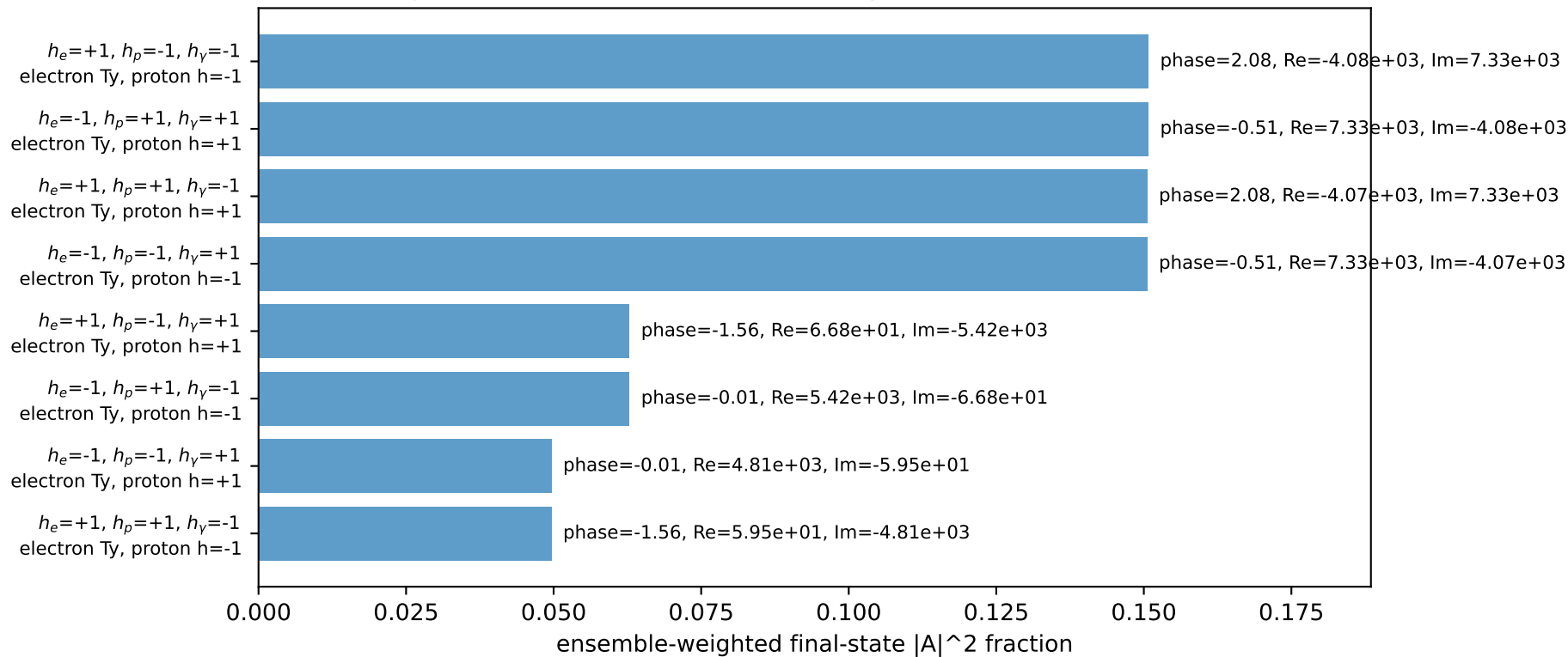
Leading initial-ensemble/final-state components (N=8, retained=82.8%)
