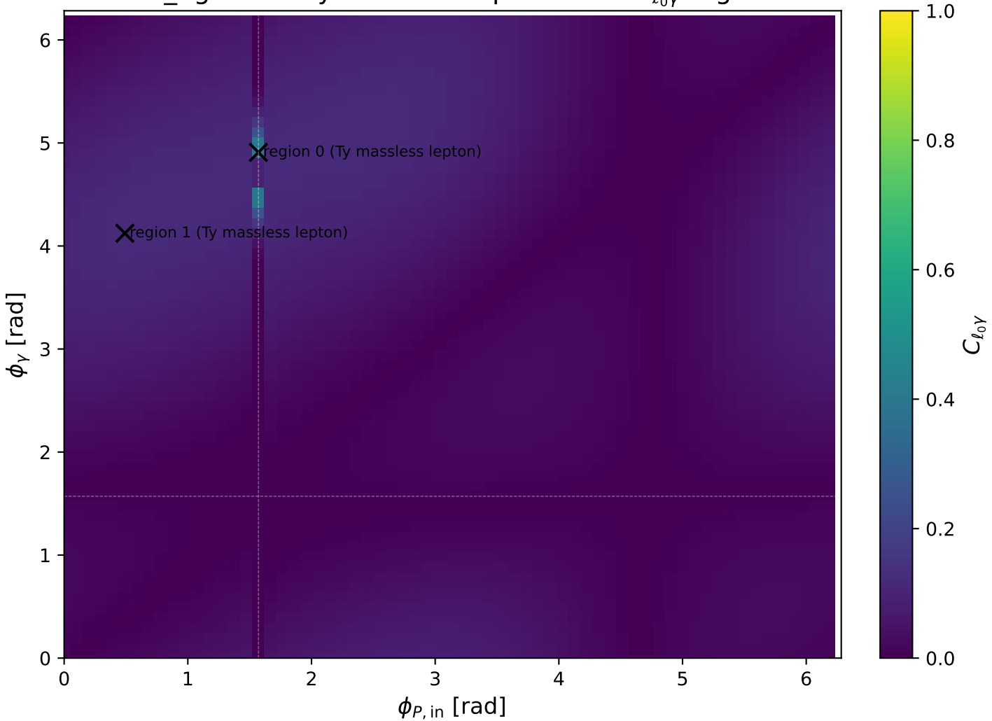
low_Egamma Ty massless lepton: max C_{\ell_0\gamma} regions
