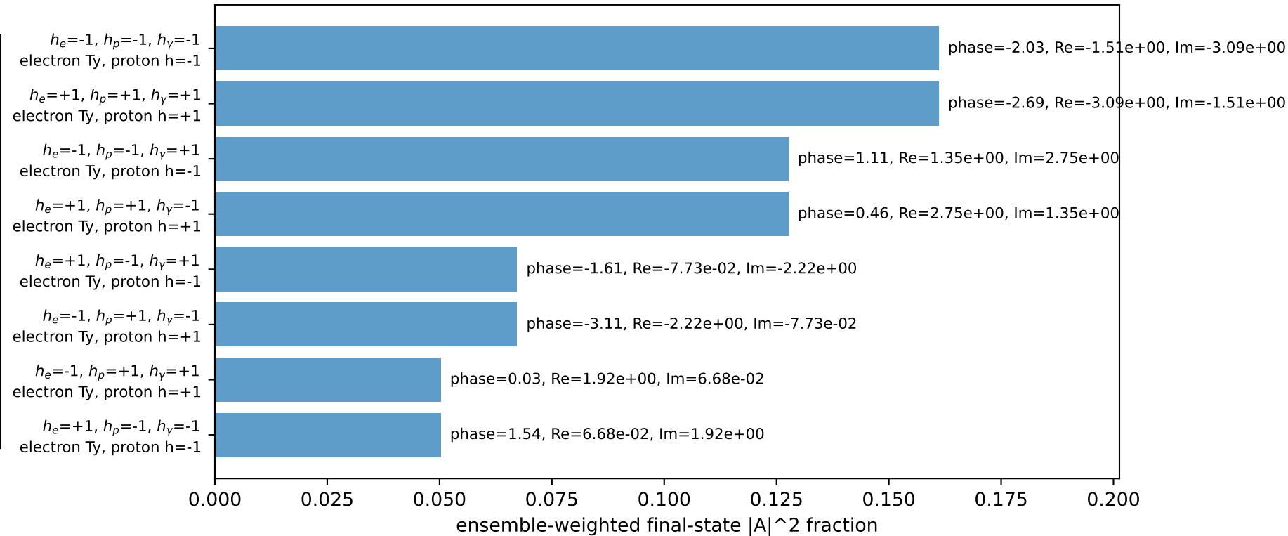
Leading initial-ensemble/final-state components (N=8, retained=81.2%)
