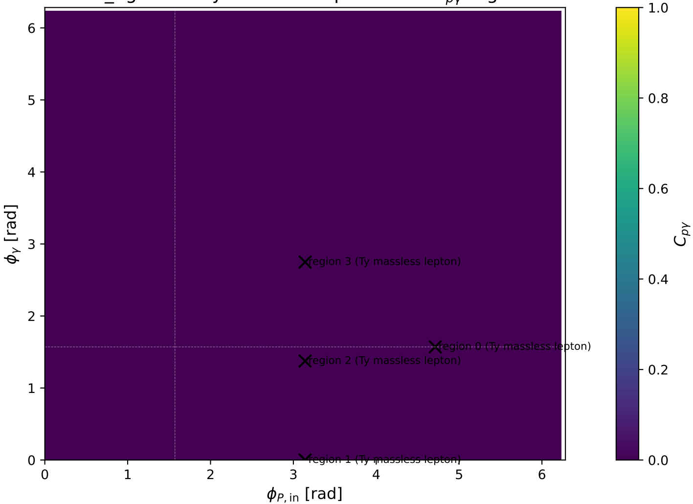
low_Egamma Ty massless lepton: max C_{p\gamma} regions
