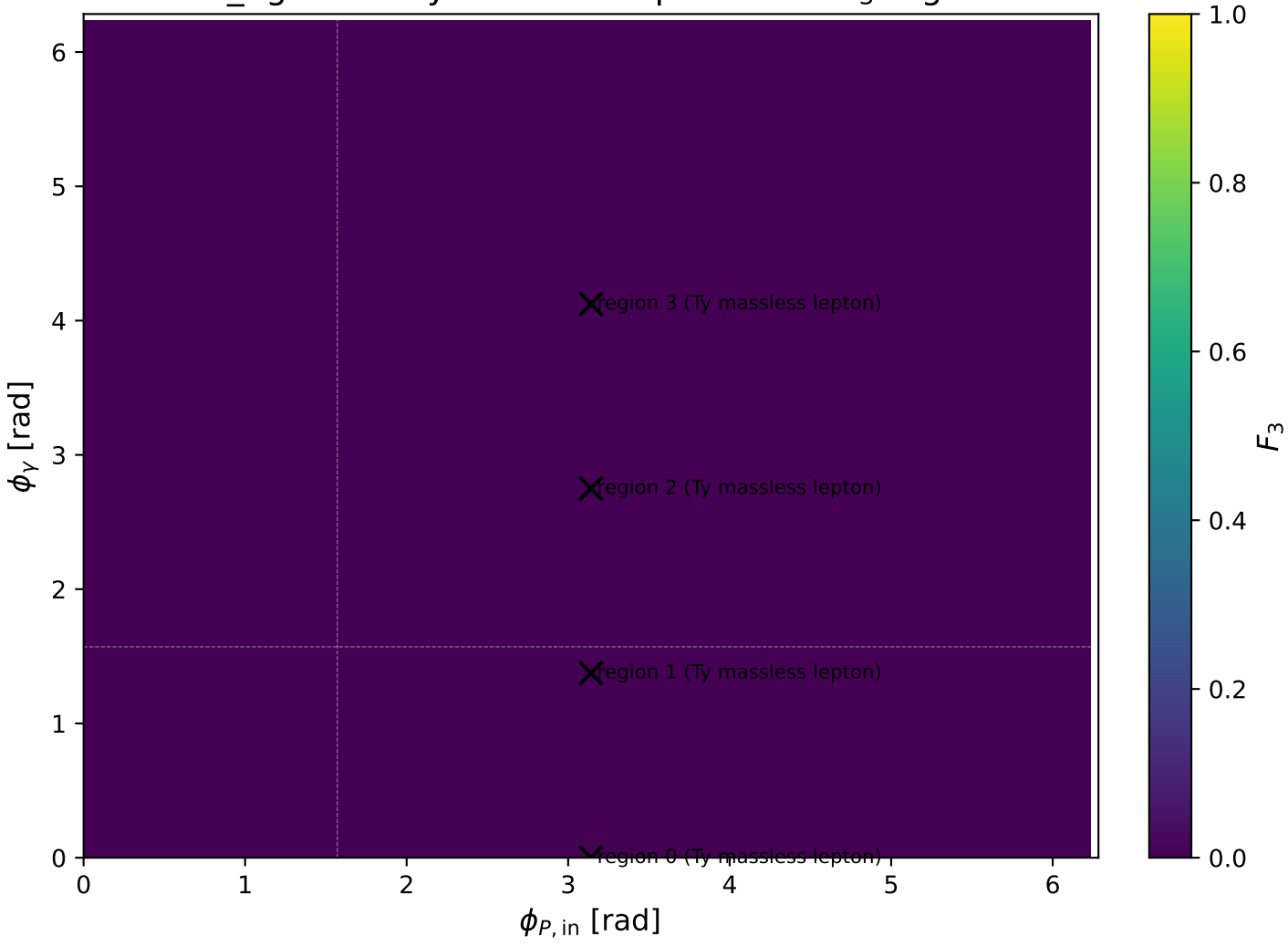
low_Egamma Ty massless lepton: max F_3 regions
