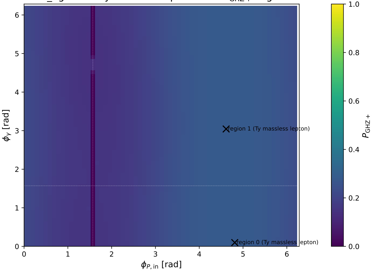
low_Egamma Ty massless lepton: max P_{\text{GHZ}+} regions
