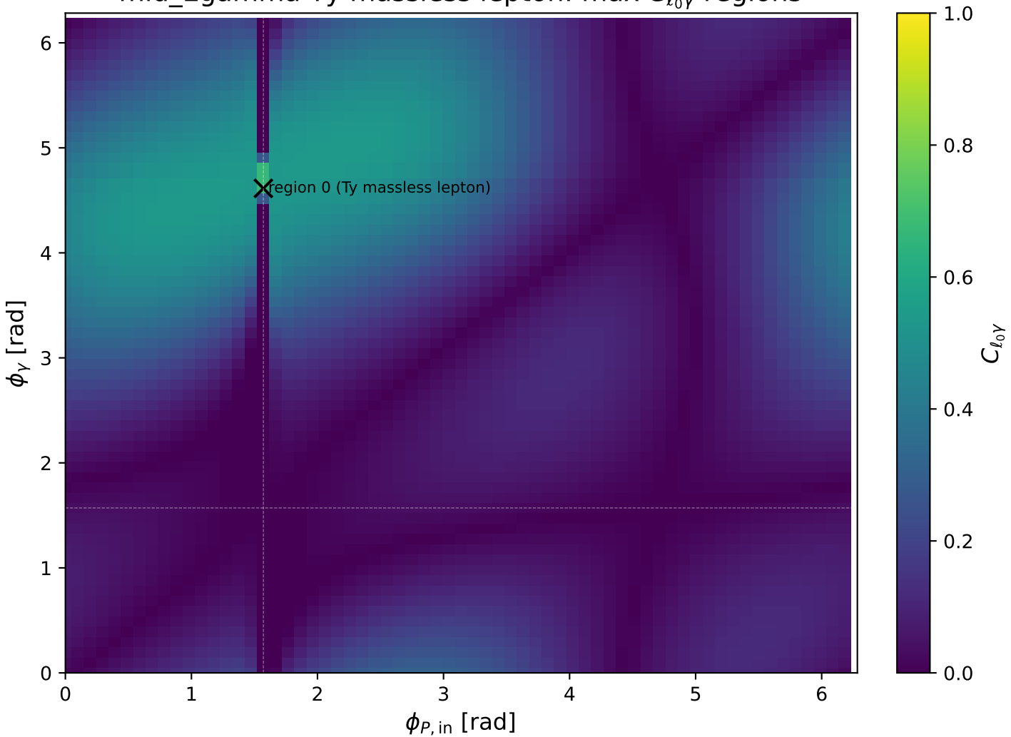
mid_Egamma Ty massless lepton: max C_{\ell_0\gamma} regions
