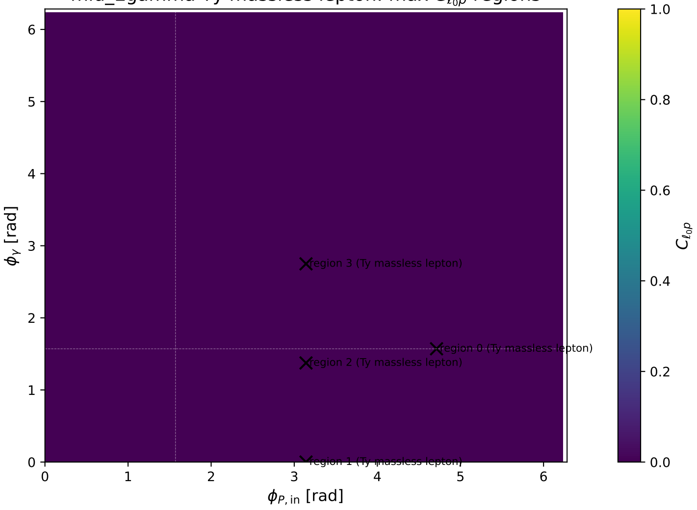
mid_Egamma Ty massless lepton: max C_{\ell_0 p} regions
