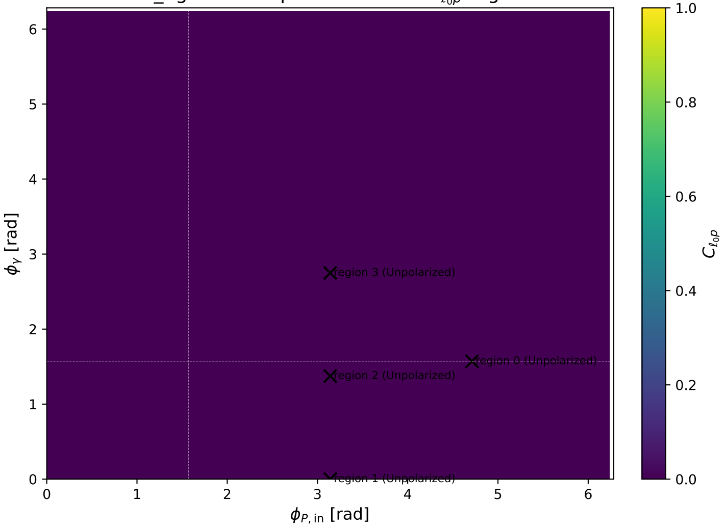
low_Egamma Unpolarized: max C_{\ell_0 p} regions
