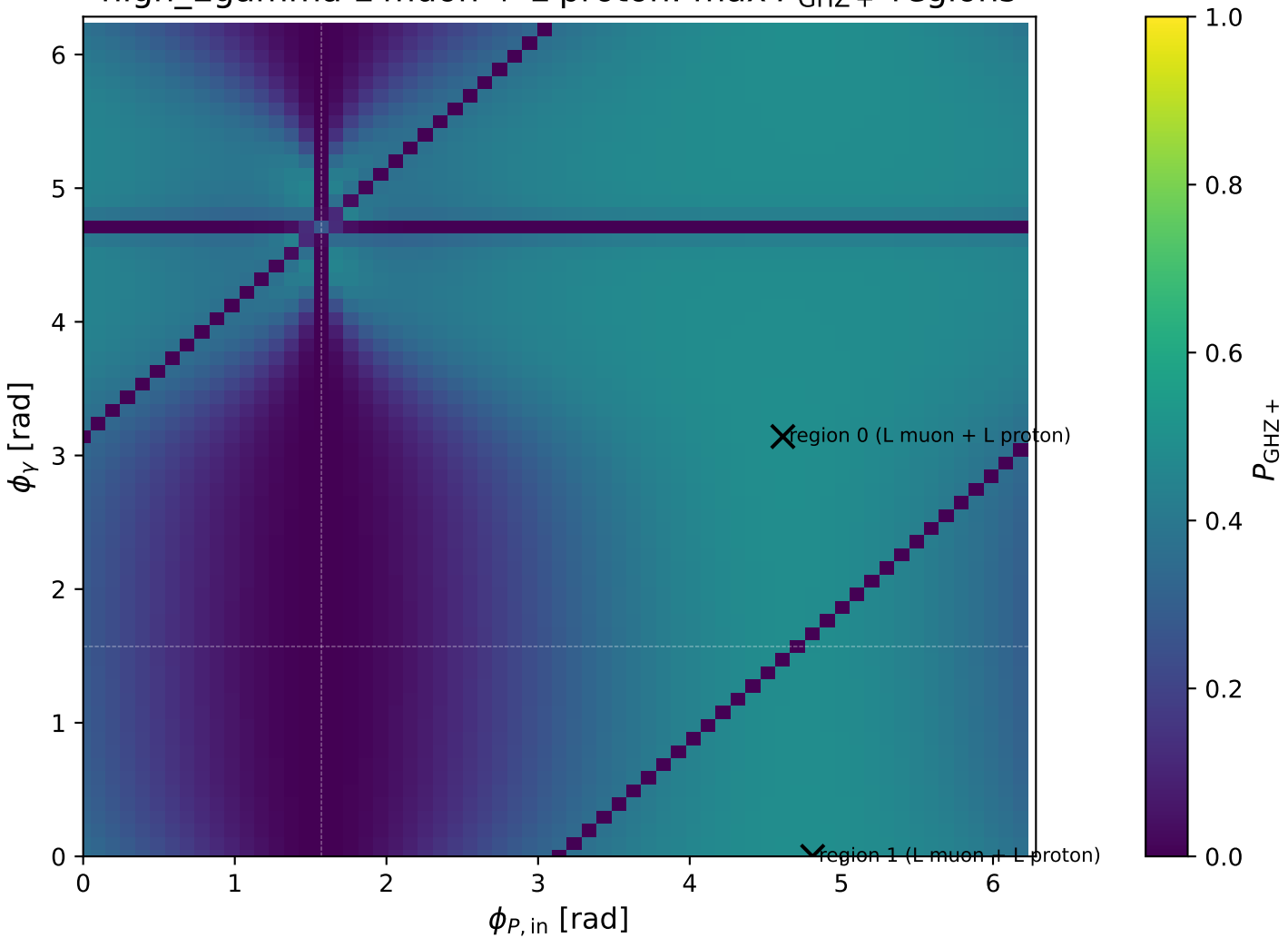
high_Egamma L muon + L proton: max P_{\text{GHZ}+} regions
