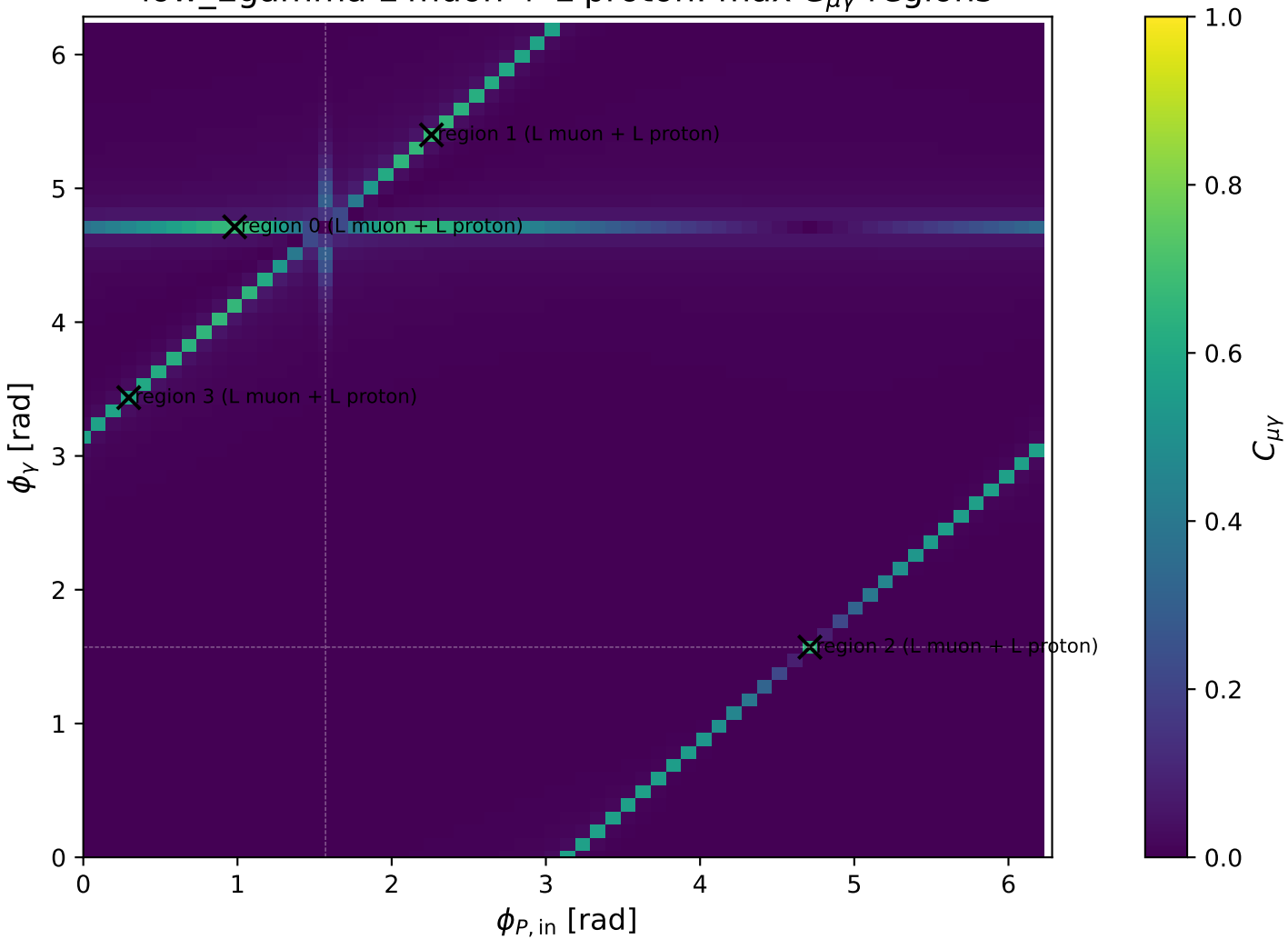
low_Egamma L muon + L proton: max C_{\mu\gamma} regions
