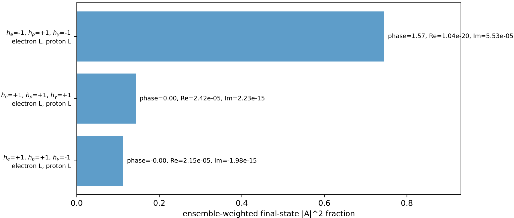
Leading initial-ensemble/final-state components (N=3, retained=100.0%)
