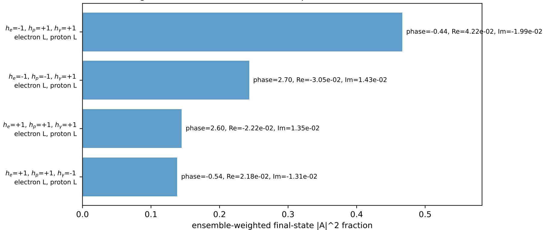
Leading initial-ensemble/final-state components (N=4, retained=99.2%)
