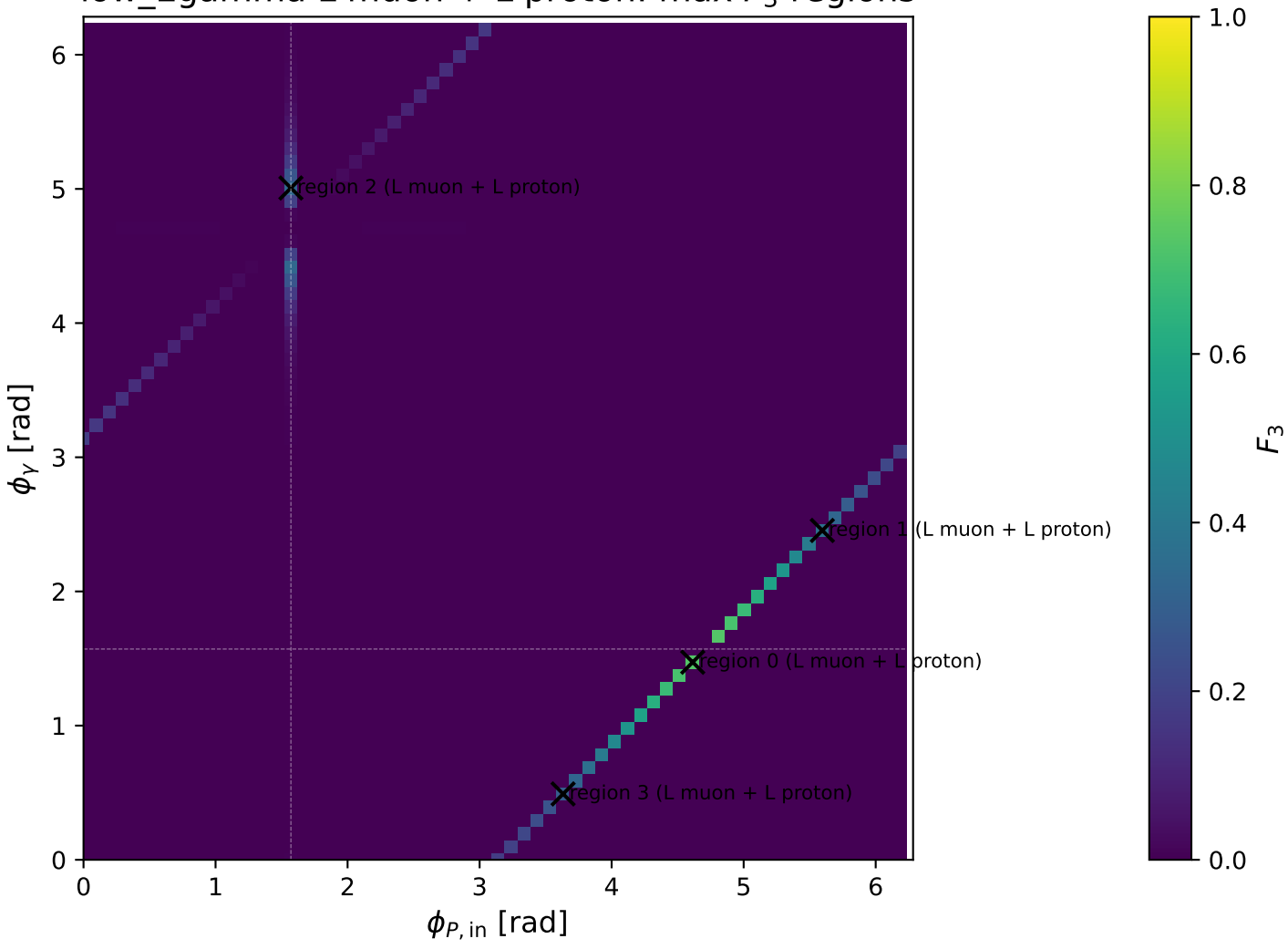
low_Egamma L muon + L proton: max F_3 regions
