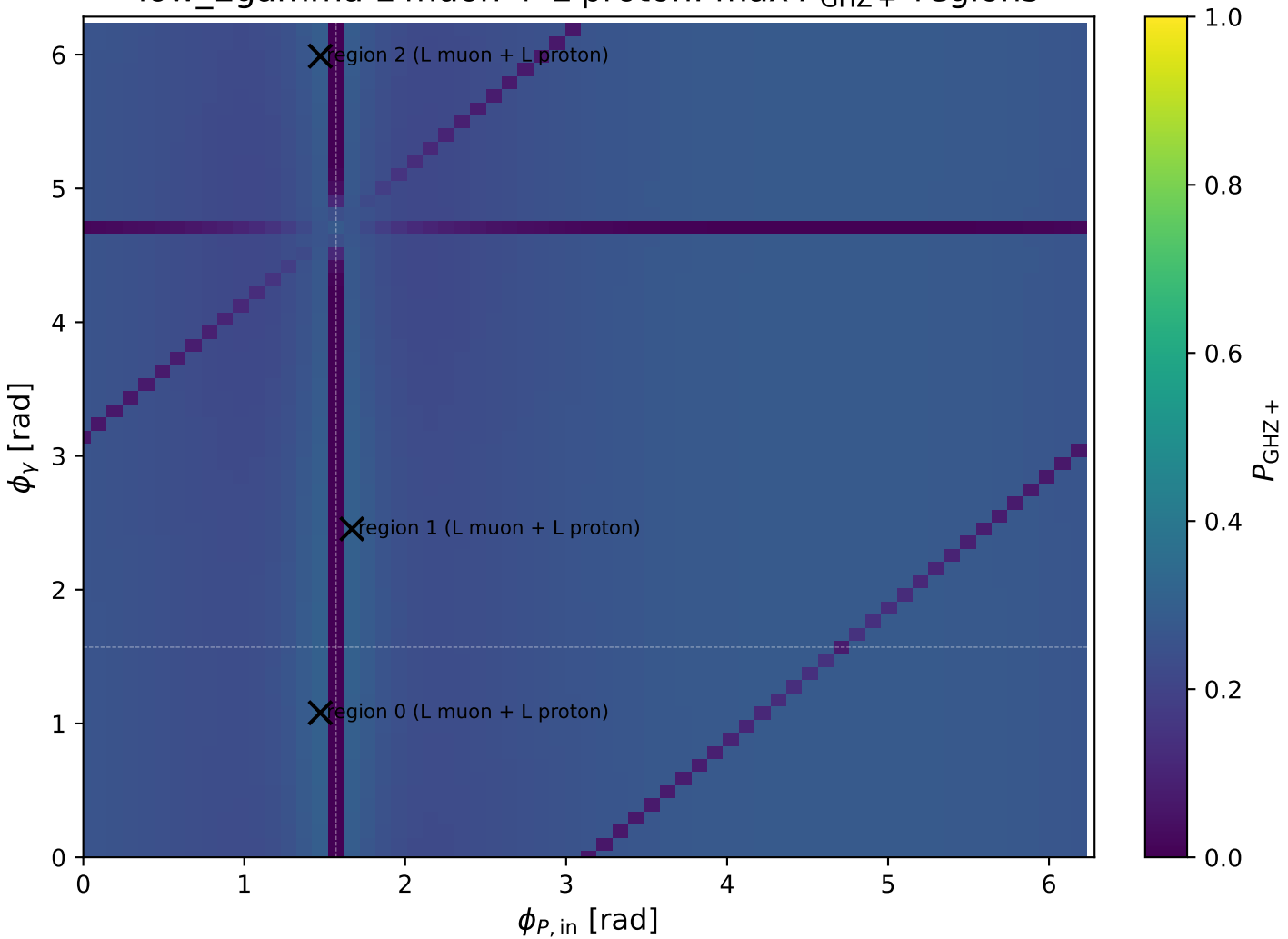
low_Egamma L muon + L proton: max P_{\text{GHZ}+} regions
