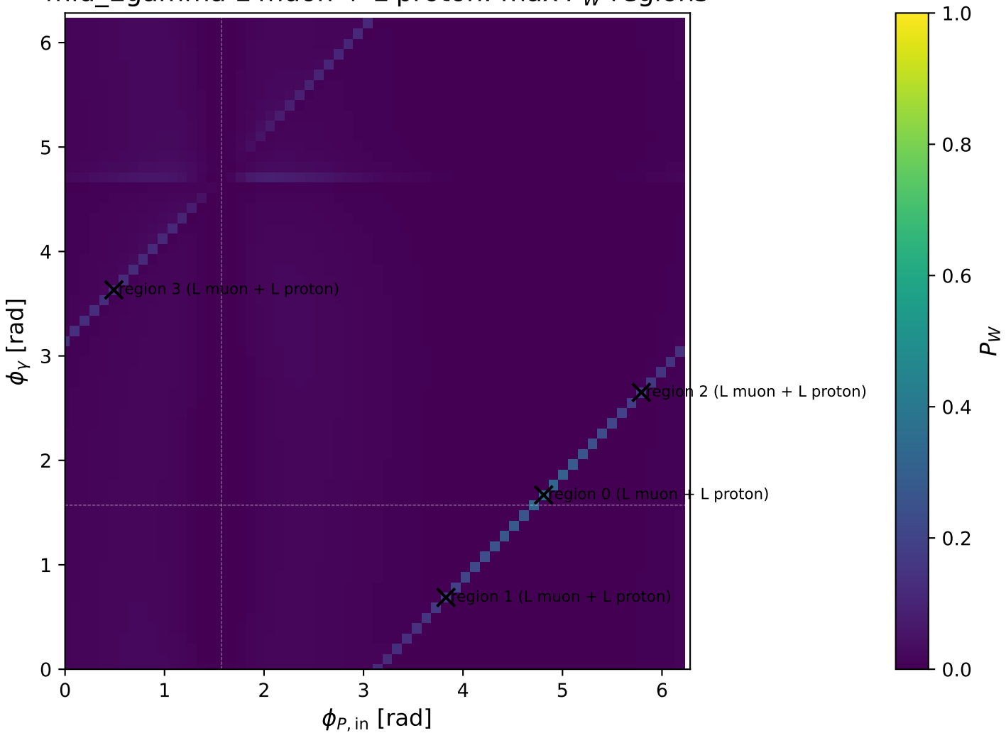
mid_Egamma L muon + L proton: max P_W regions
