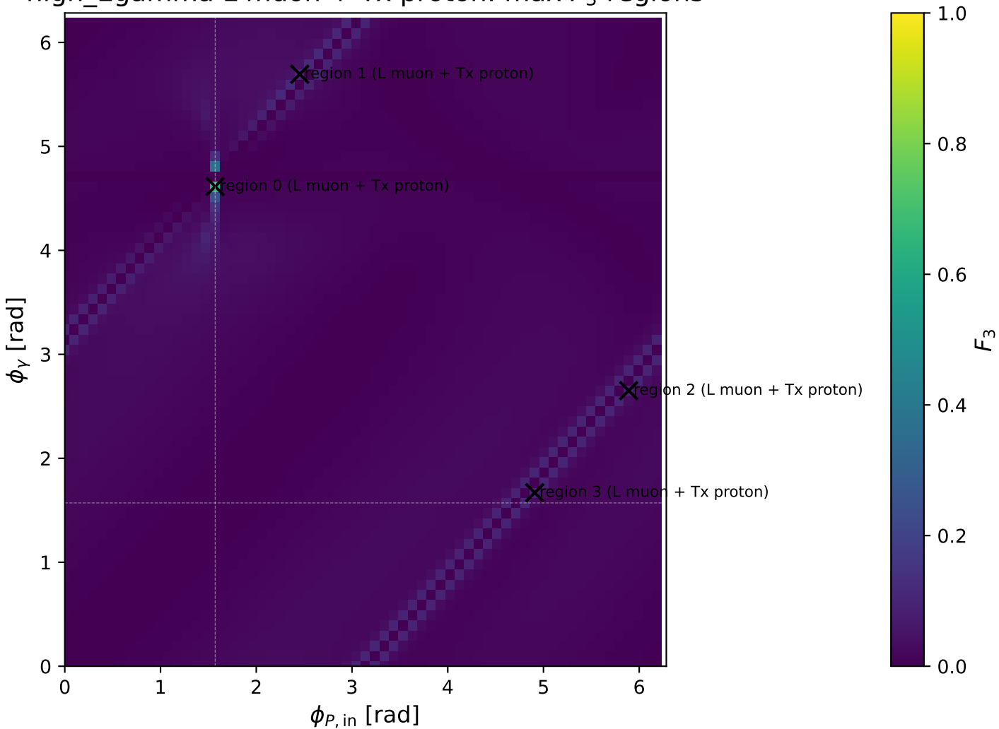
high_Egamma L muon + Tx proton: max F_3 regions
