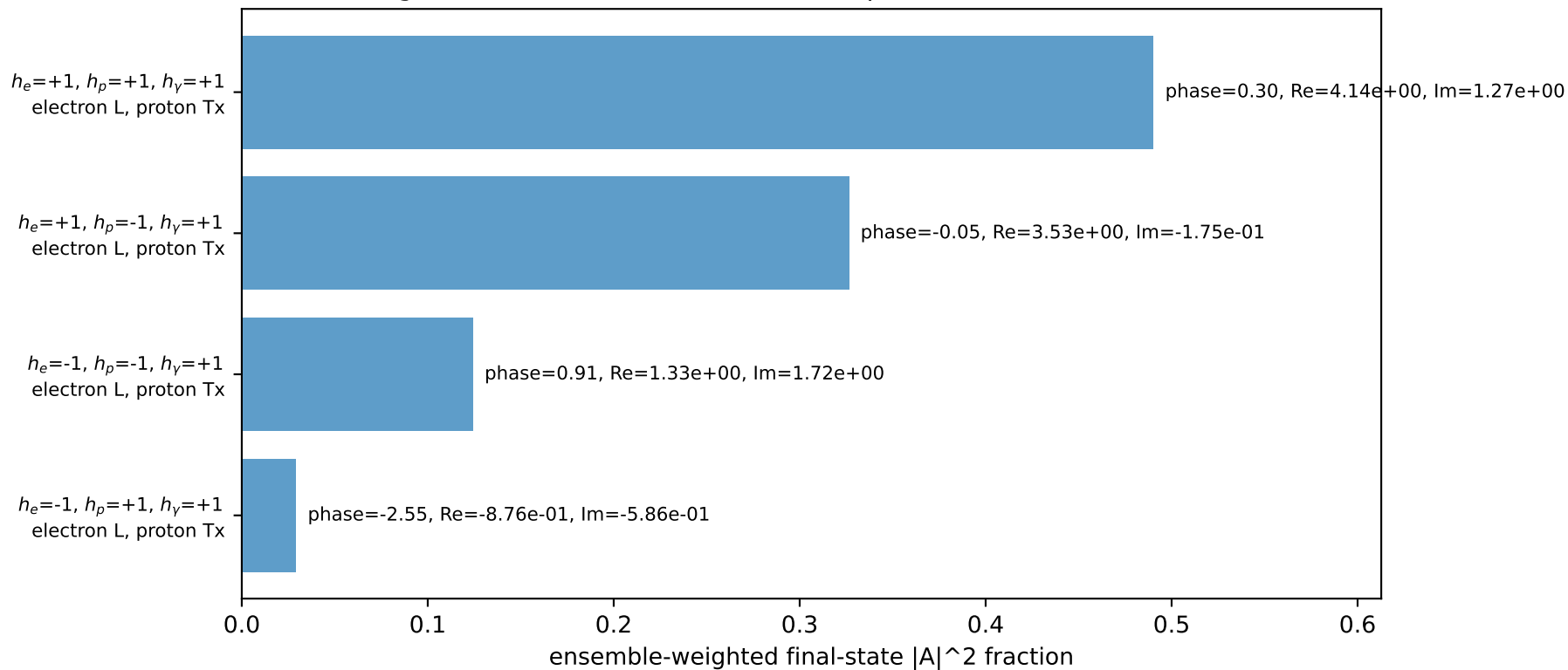
Leading initial-ensemble/final-state components (N=4, retained=97.0%)
