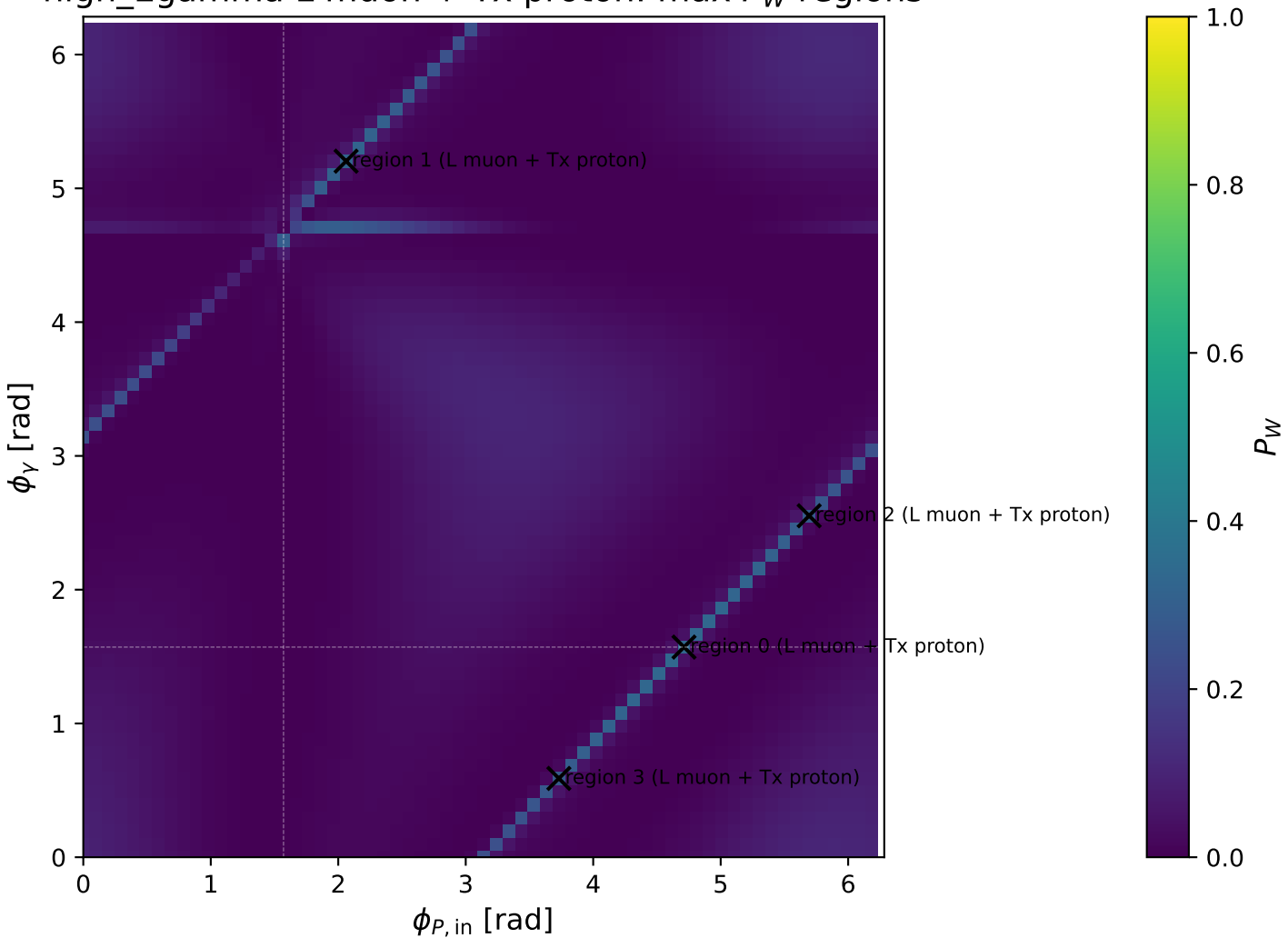
high_Egamma L muon + Tx proton: max P_W regions
