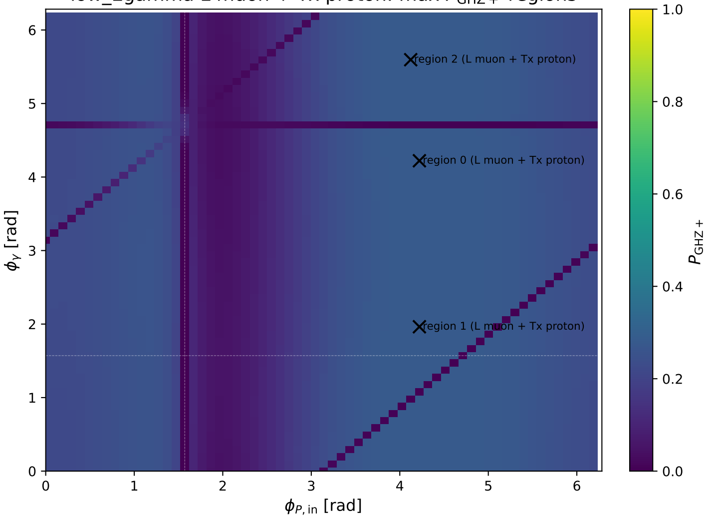
low_Egamma L muon + Tx proton: max P_{\text{GHZ}+} regions
