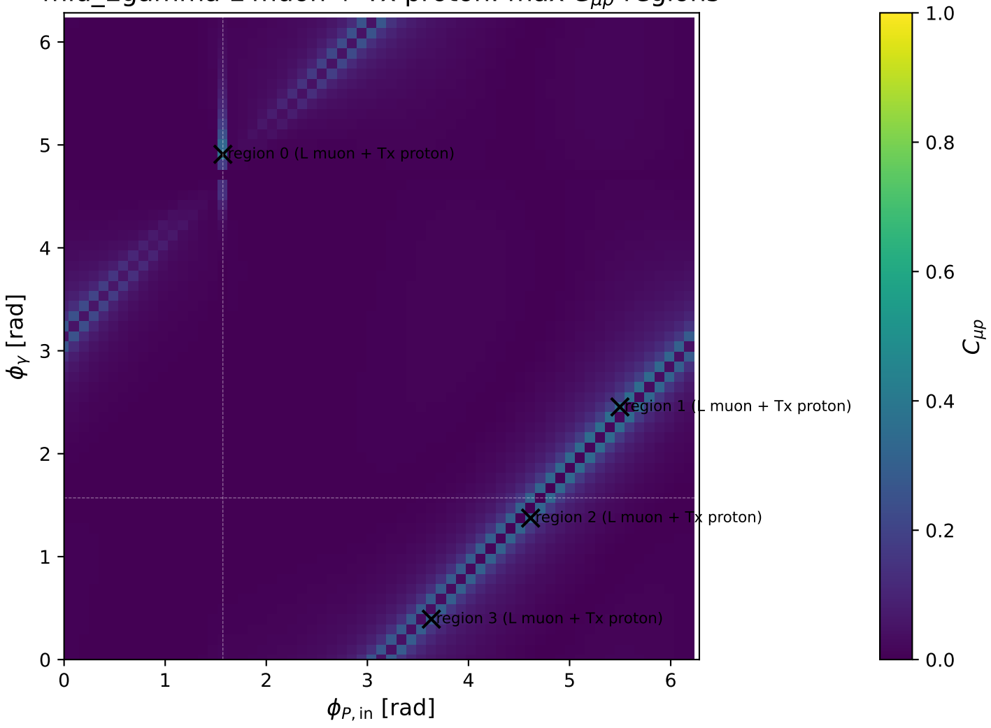
mid_Egamma L muon + Tx proton: max C_{\mu p} regions
