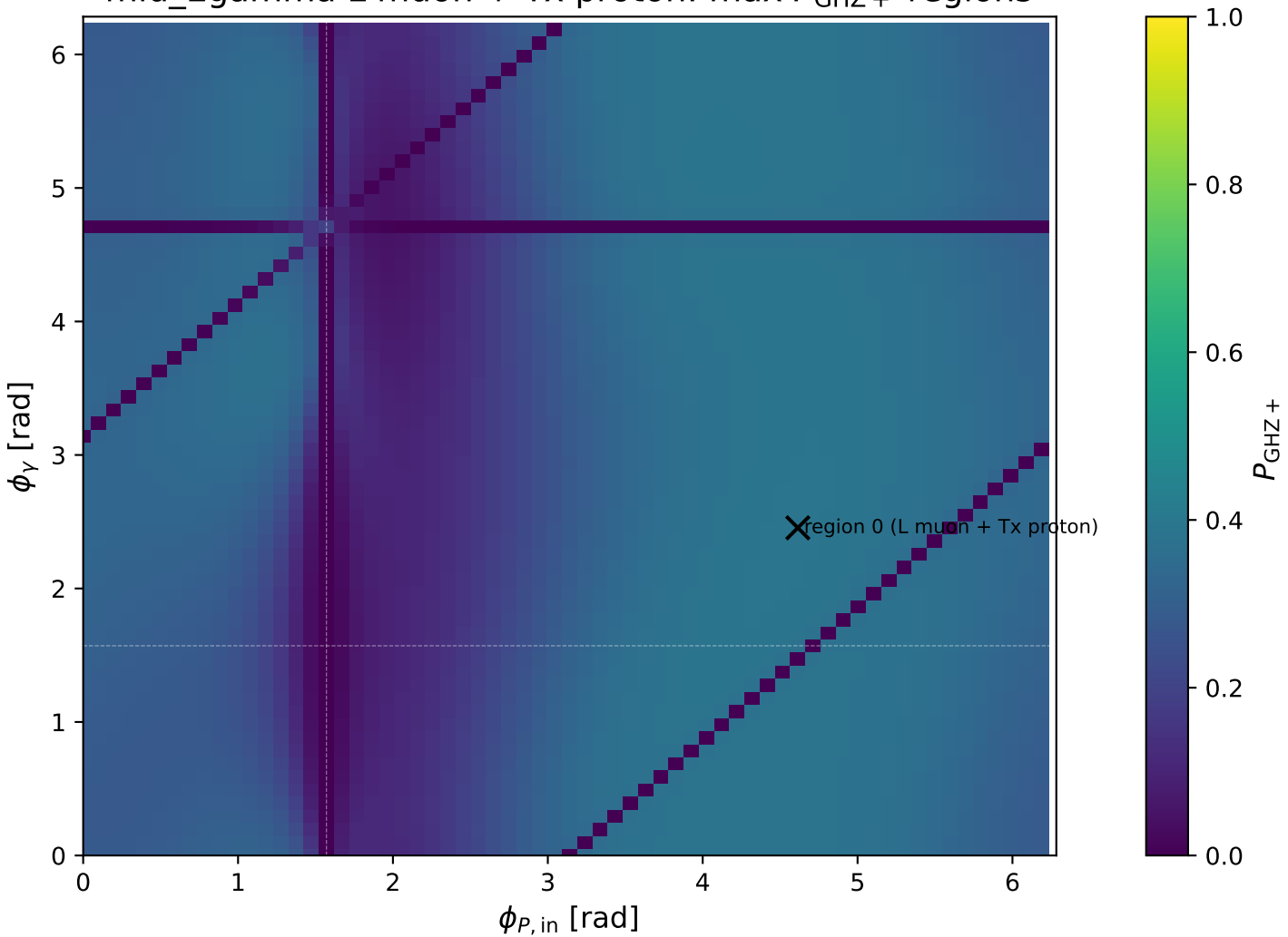
mid_Egamma L muon + Tx proton: max P_{\text{GHZ}+} regions
