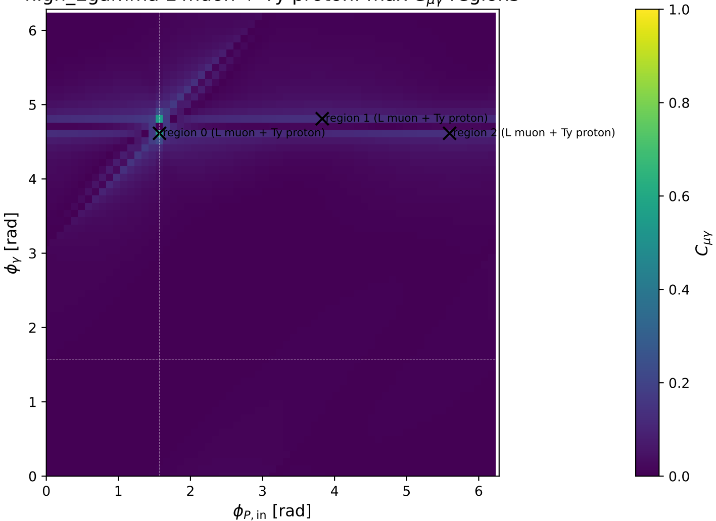
high_Egamma L muon + Ty proton: max C_{\mu\gamma} regions
