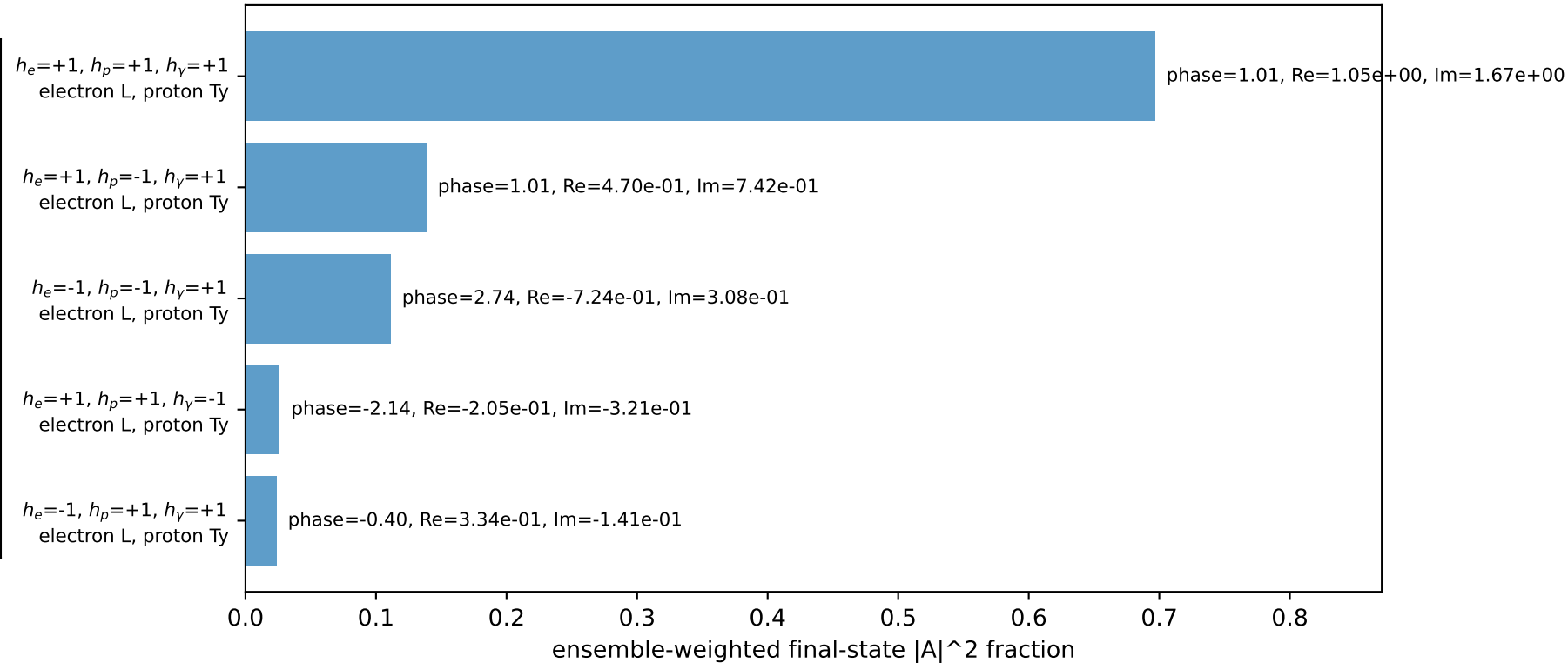
Leading initial-ensemble/final-state components (N=5, retained=99.5%)
