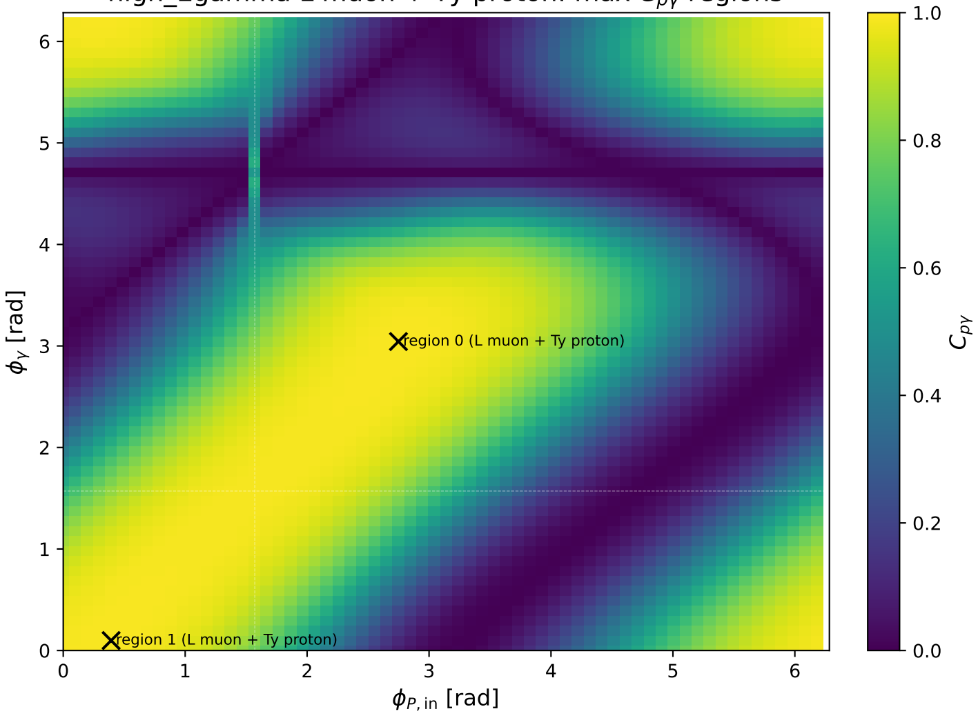
high_Egamma L muon + Ty proton: max C_{p\gamma} regions
