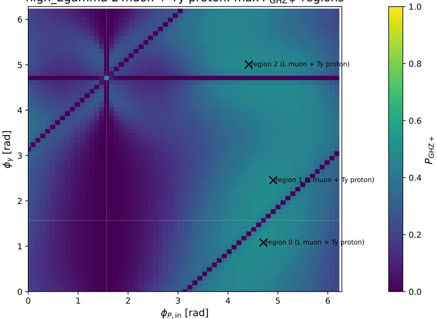
high_Egamma L muon + Ty proton: max P_{\text{GHZ}} + regions
