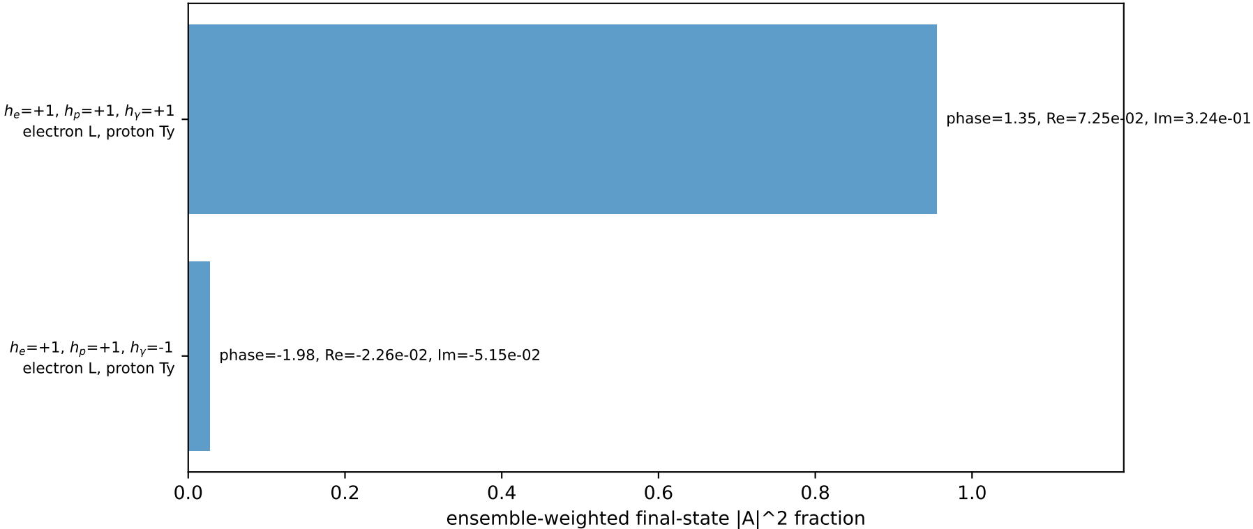
Leading initial-ensemble/final-state components (N=2, retained=98.2%)
