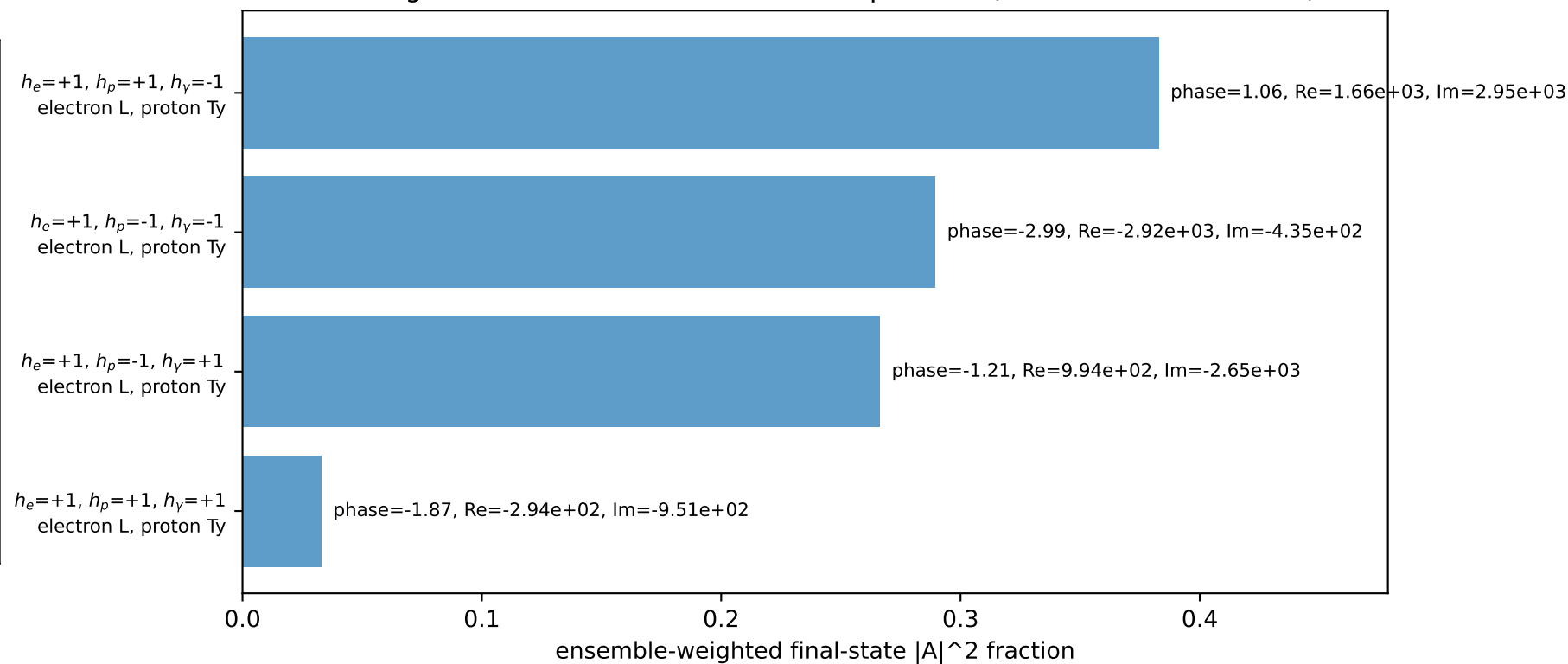
Leading initial-ensemble/final-state components (N=4, retained=97.2%)
