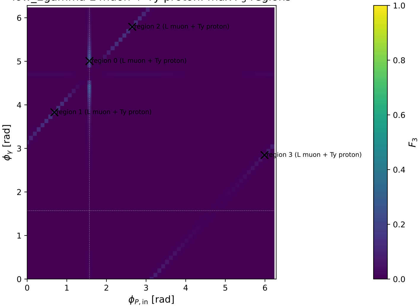
low_Egamma L muon + Ty proton: max F_3 regions
