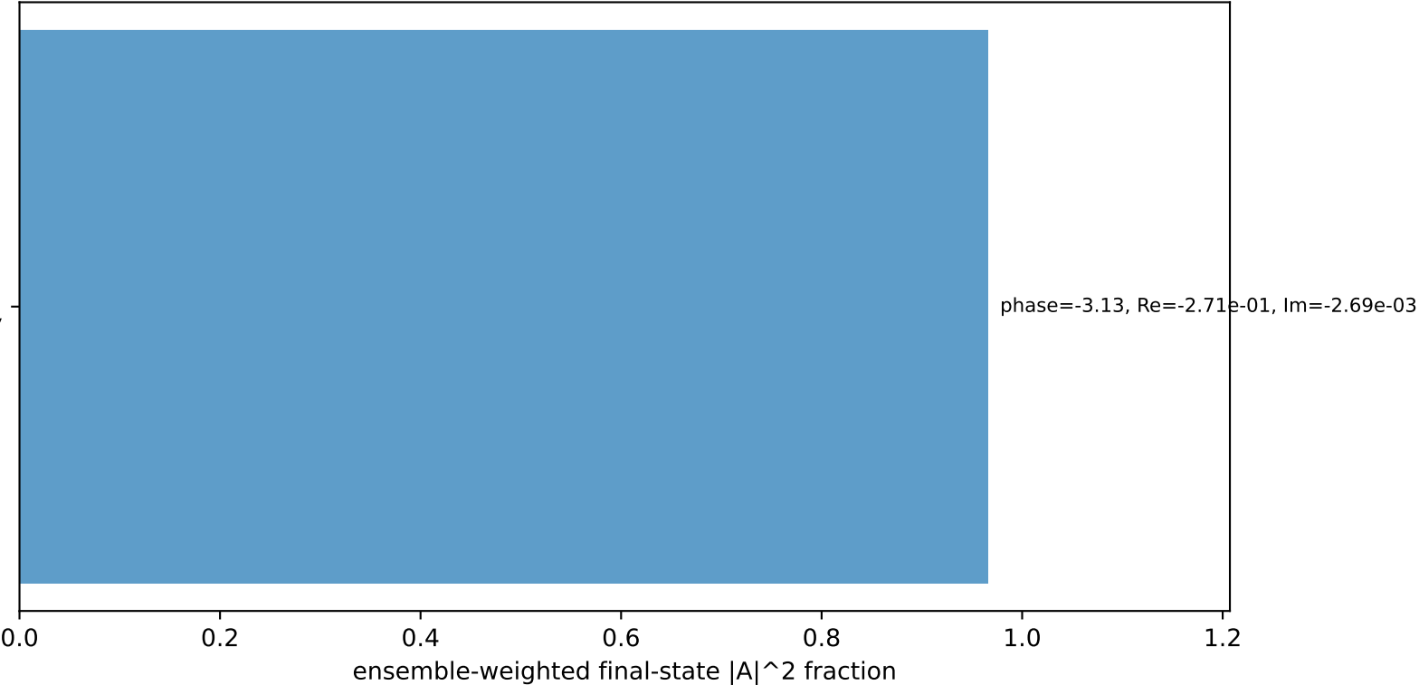
Leading initial-ensemble/final-state components (N=1, retained=96.6%)
