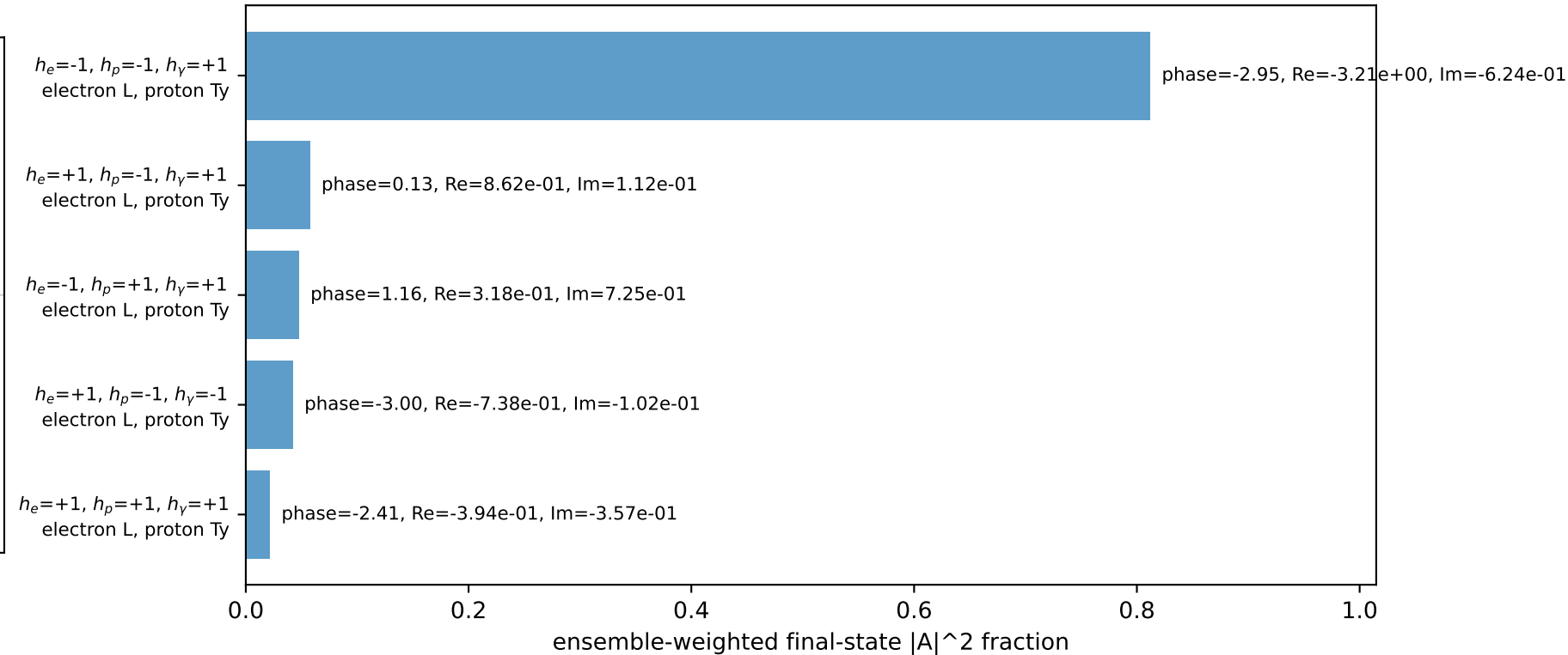
Leading initial-ensemble/final-state components (N=5, retained=98.1%)
