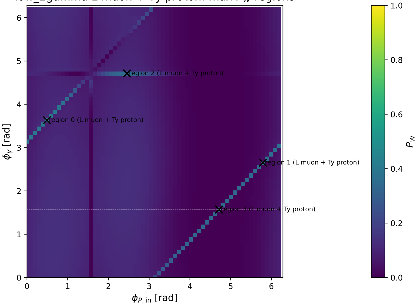
low_Egamma L muon + Ty proton: max P_W regions
