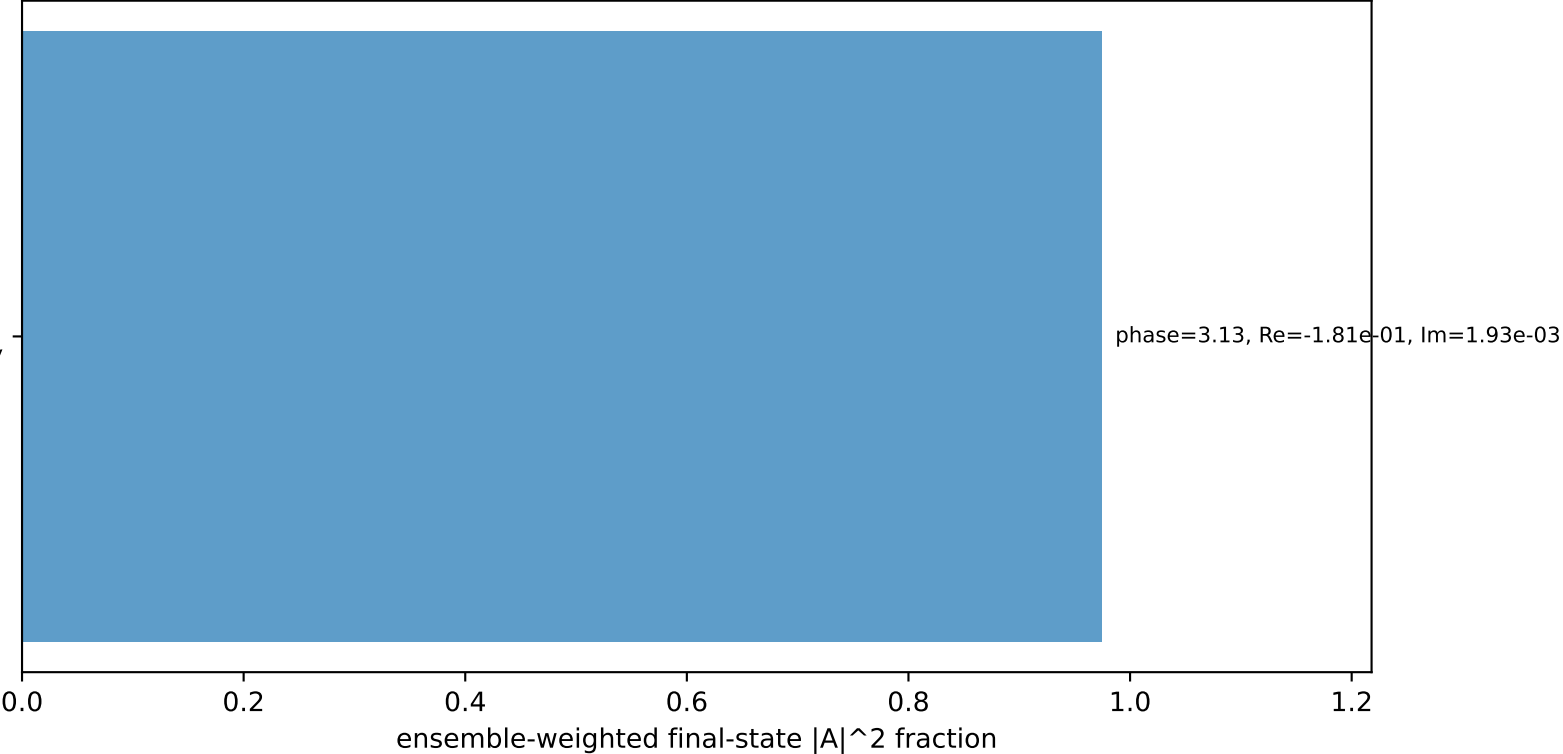
Leading initial-ensemble/final-state components (N=1, retained=97.4%)
