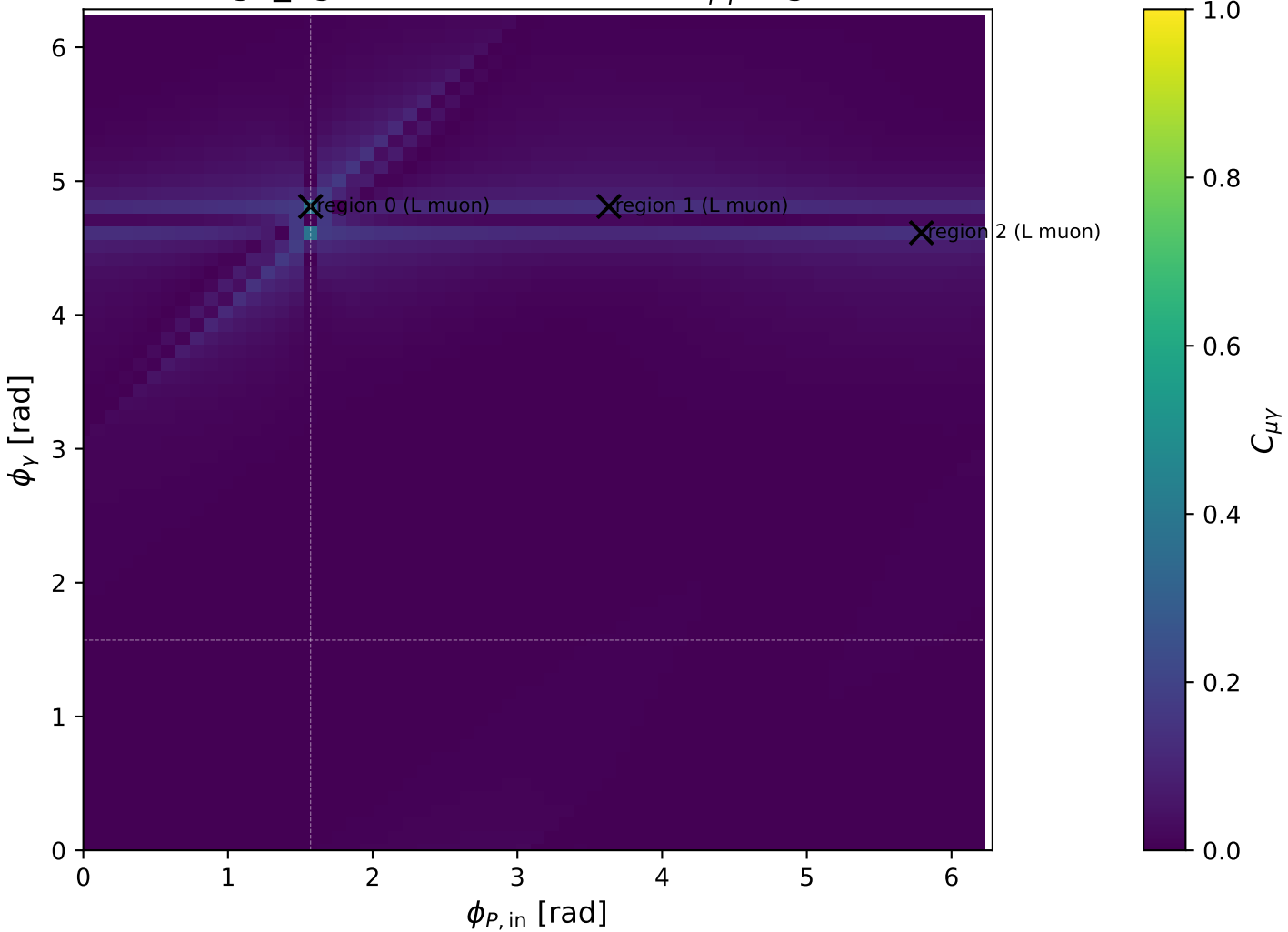
high_Egamma L muon: max C_{\mu\gamma} regions
