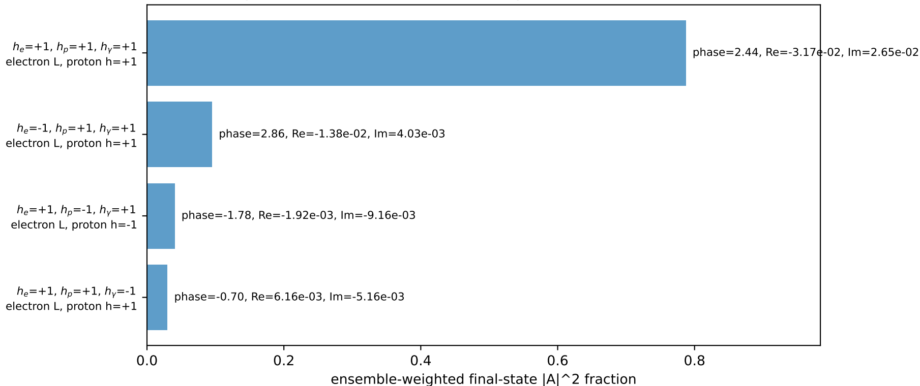
Leading initial-ensemble/final-state components (N=4, retained=95.2%)
