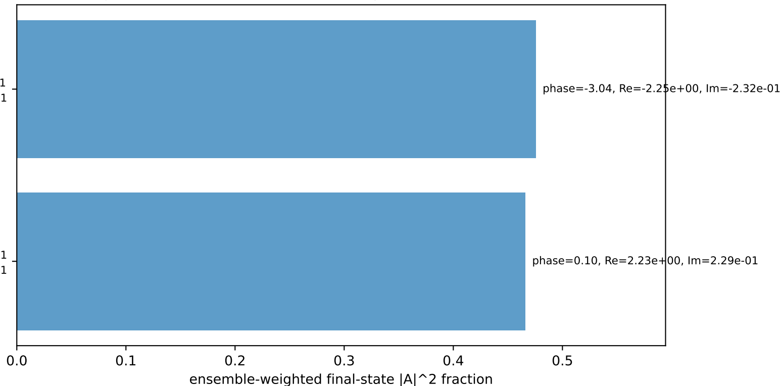
Leading initial-ensemble/final-state components (N=2, retained=94.2%)
