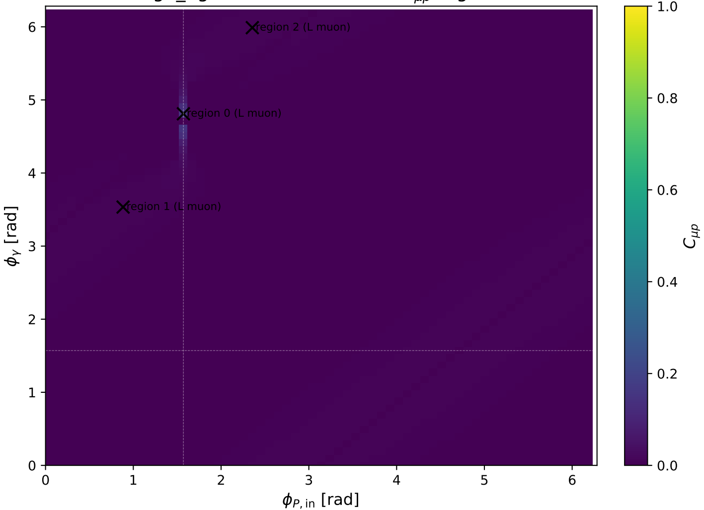
high_Egamma L muon: max C_{\mu p} regions
