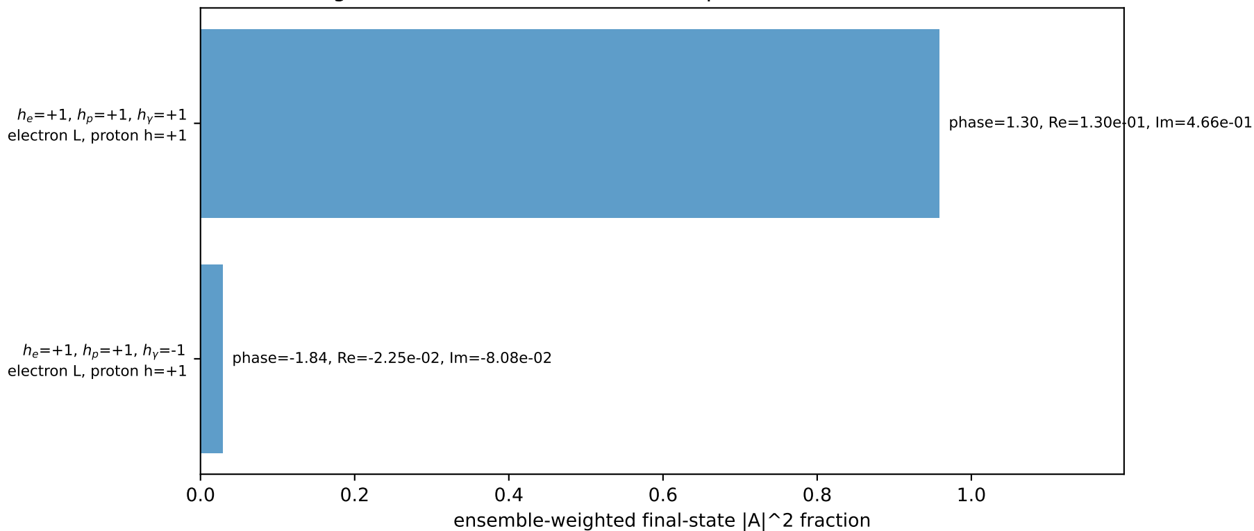
Leading initial-ensemble/final-state components (N=2, retained=98.7%)
