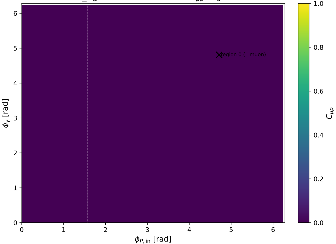
low_Egamma L muon: max C_{\mu p} regions
