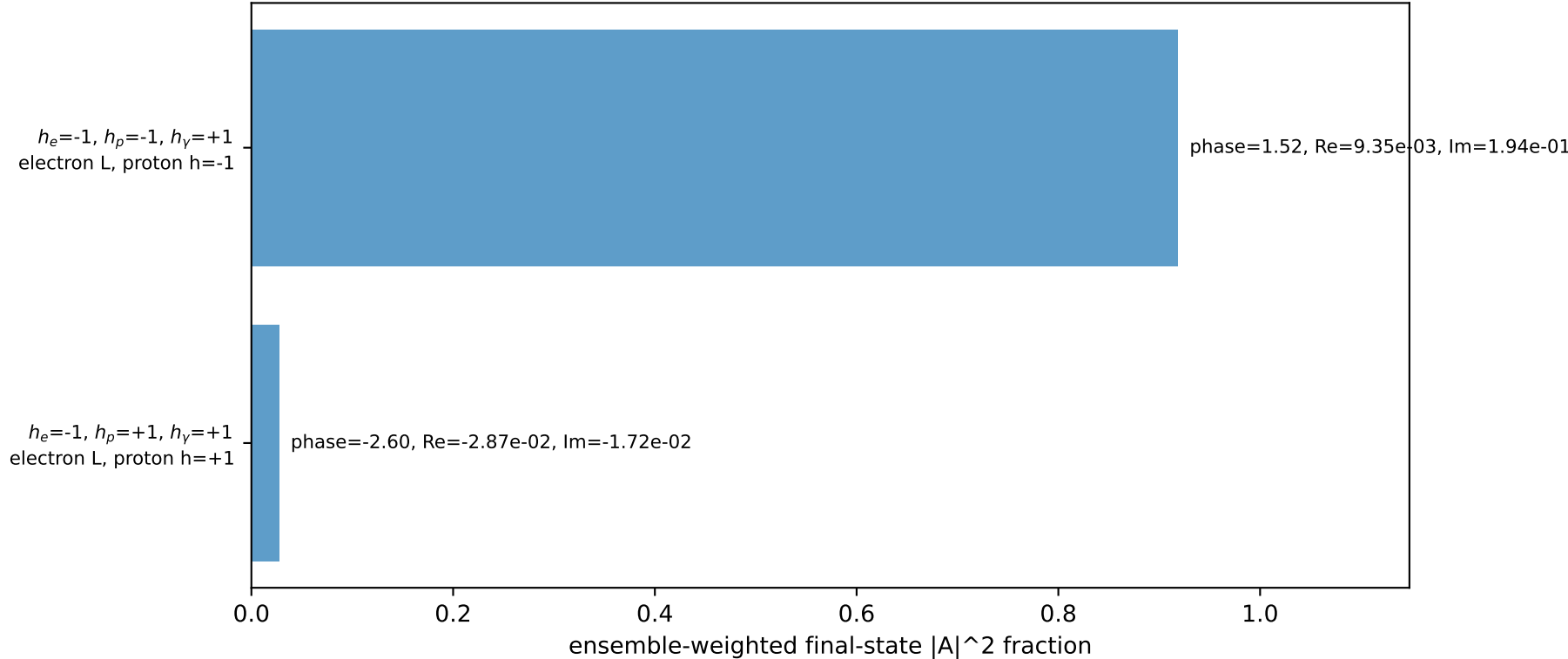
Leading initial-ensemble/final-state components (N=2, retained=94.6%)
