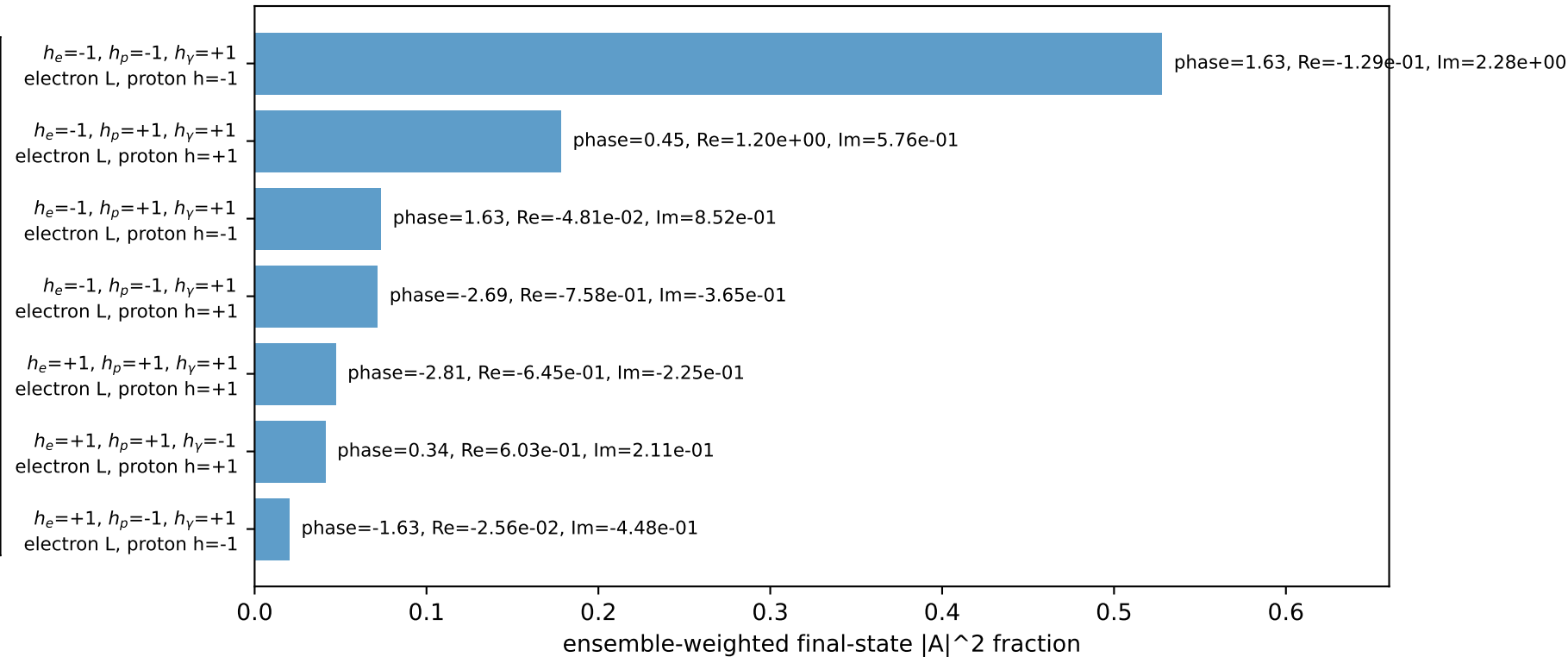
Leading initial-ensemble/final-state components (N=7, retained=96.0%)
