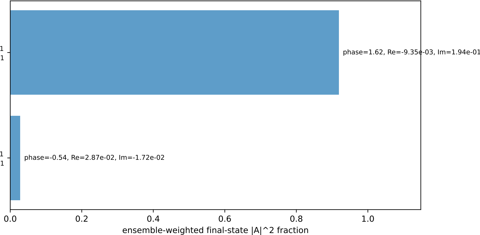
Leading initial-ensemble/final-state components (N=2, retained=94.6%)
