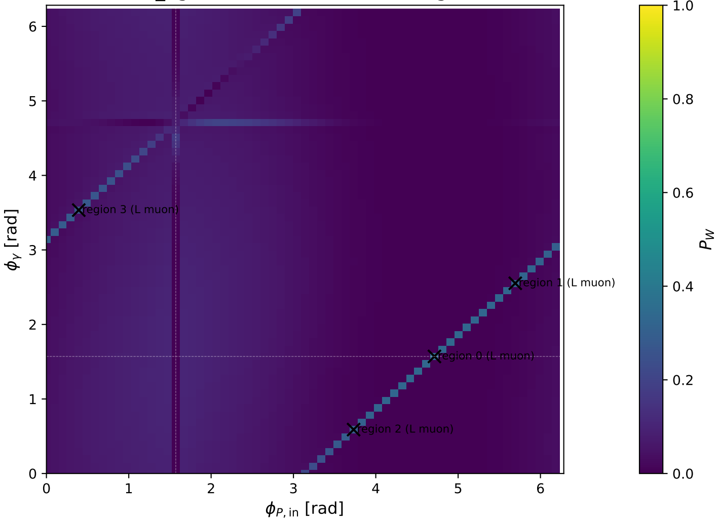
low_Egamma L muon: max P_W regions
