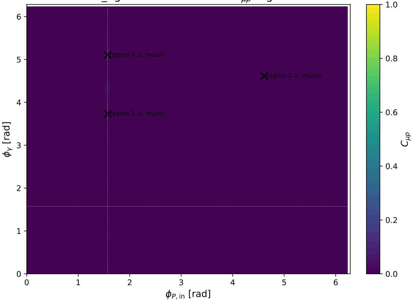
mid_Egamma L muon: max C_{\mu p} regions
