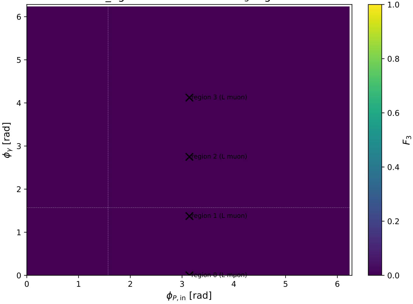
mid_Egamma L muon: max F_3 regions
