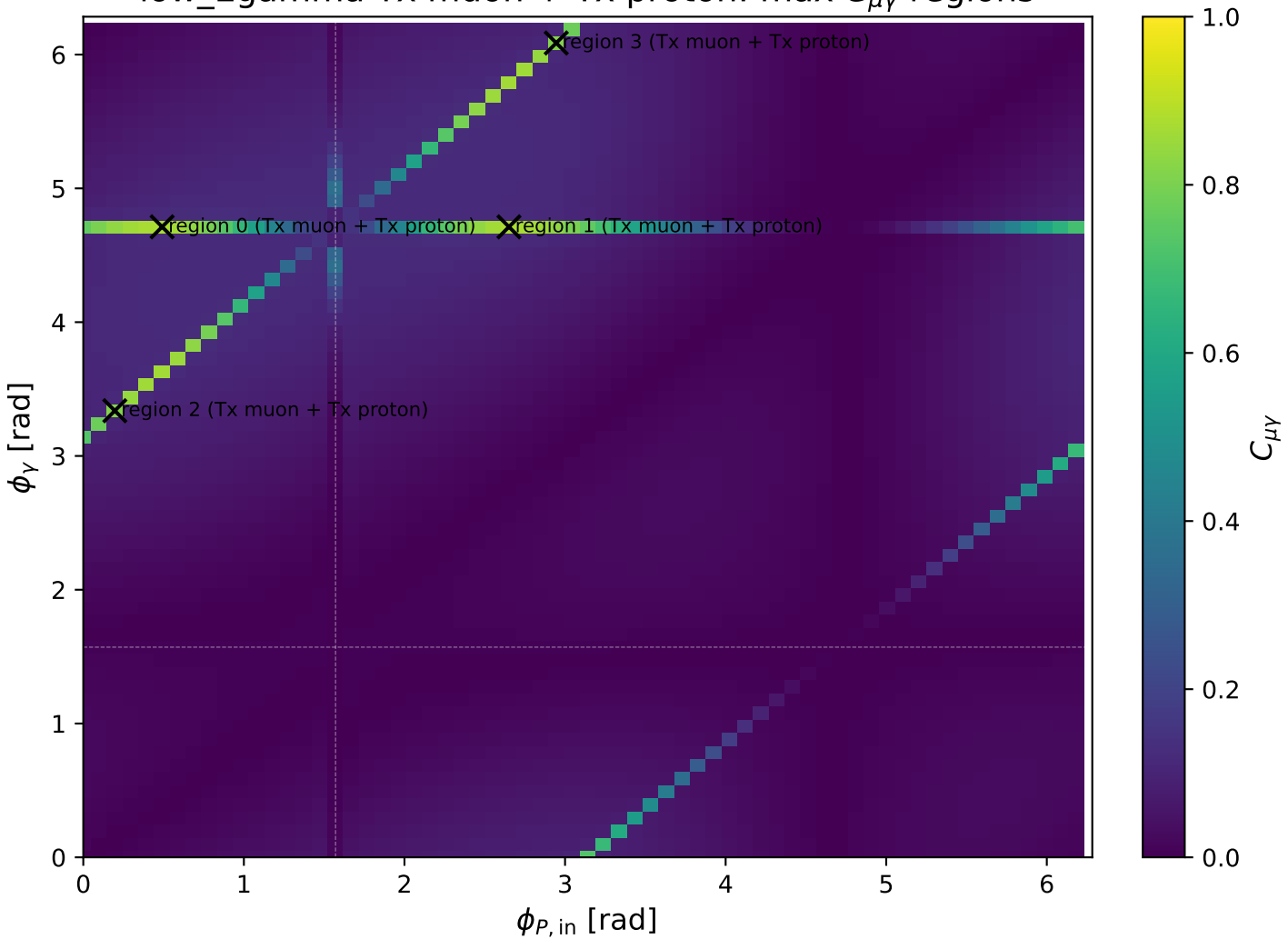
low_Egamma Tx muon + Tx proton: max C_{\mu\gamma} regions
