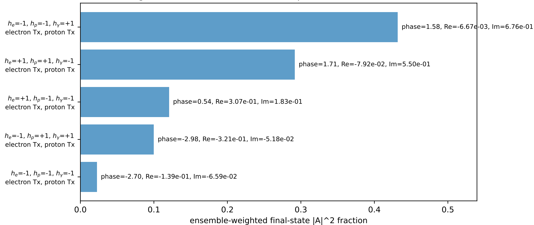
Leading initial-ensemble/final-state components (N=5, retained=96.6%)
