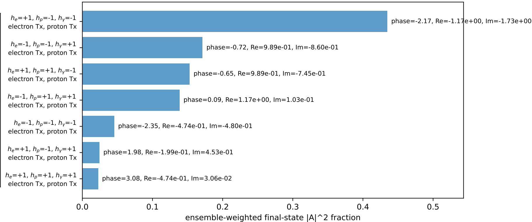
Leading initial-ensemble/final-state components (N=7, retained=99.0%)
