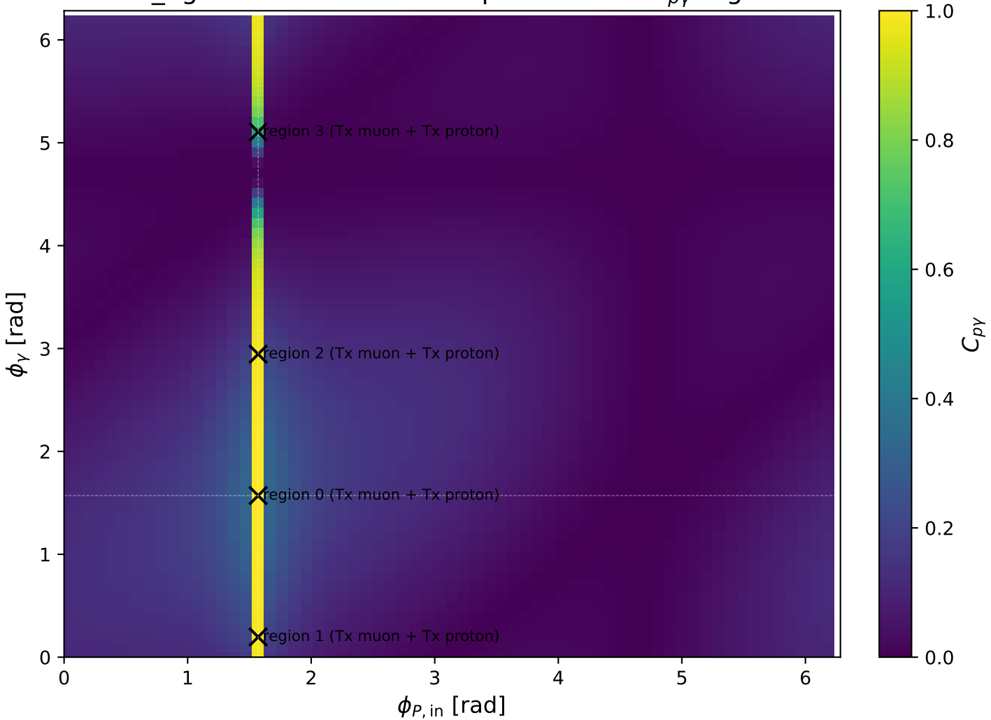
low_Egamma Tx muon + Tx proton: max C_{p\gamma} regions
