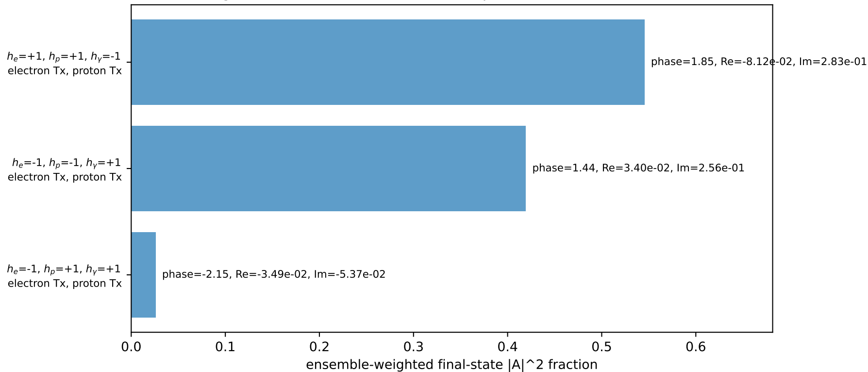
Leading initial-ensemble/final-state components (N=3, retained=99.0%)
