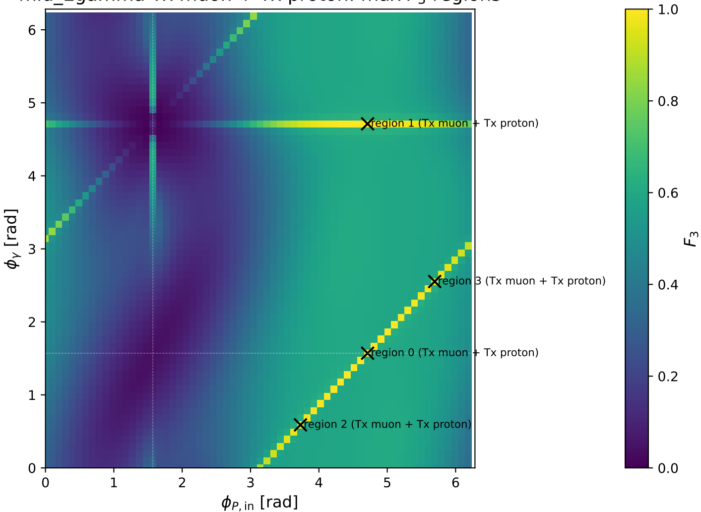
mid_Egamma Tx muon + Tx proton: max F_3 regions
