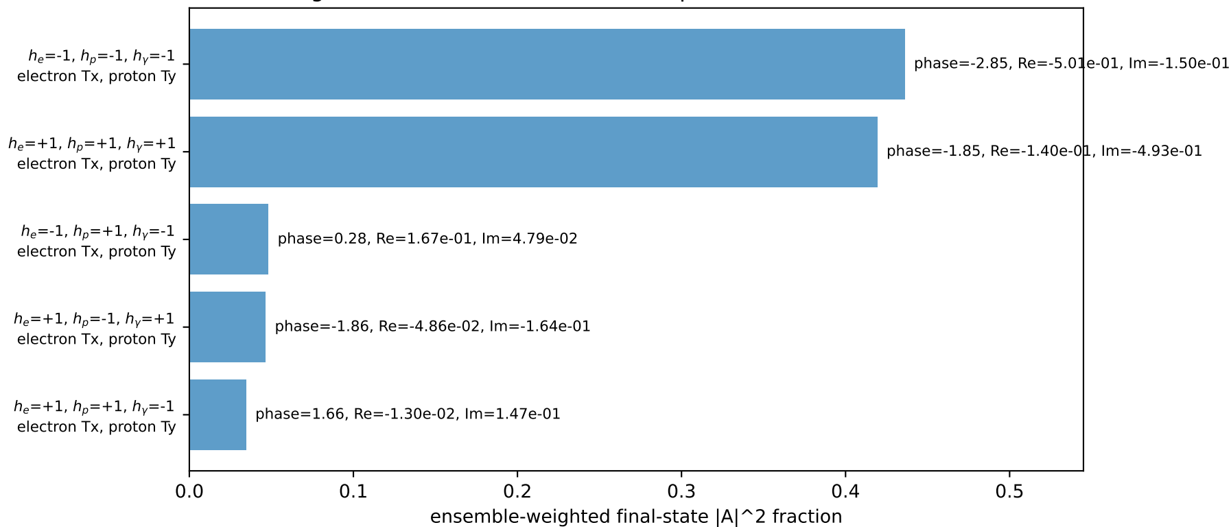
Leading initial-ensemble/final-state components (N=5, retained=98.4%)
