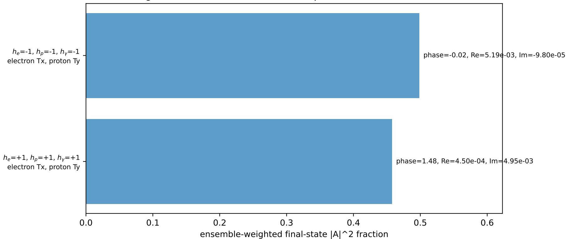
Leading initial-ensemble/final-state components (N=2, retained=95.6%)
