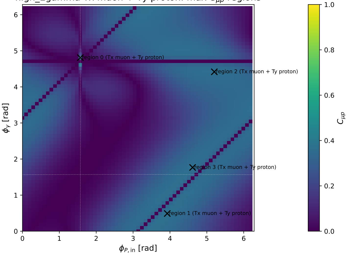
high_Egamma Tx muon + Ty proton: max C_{\mu p} regions
