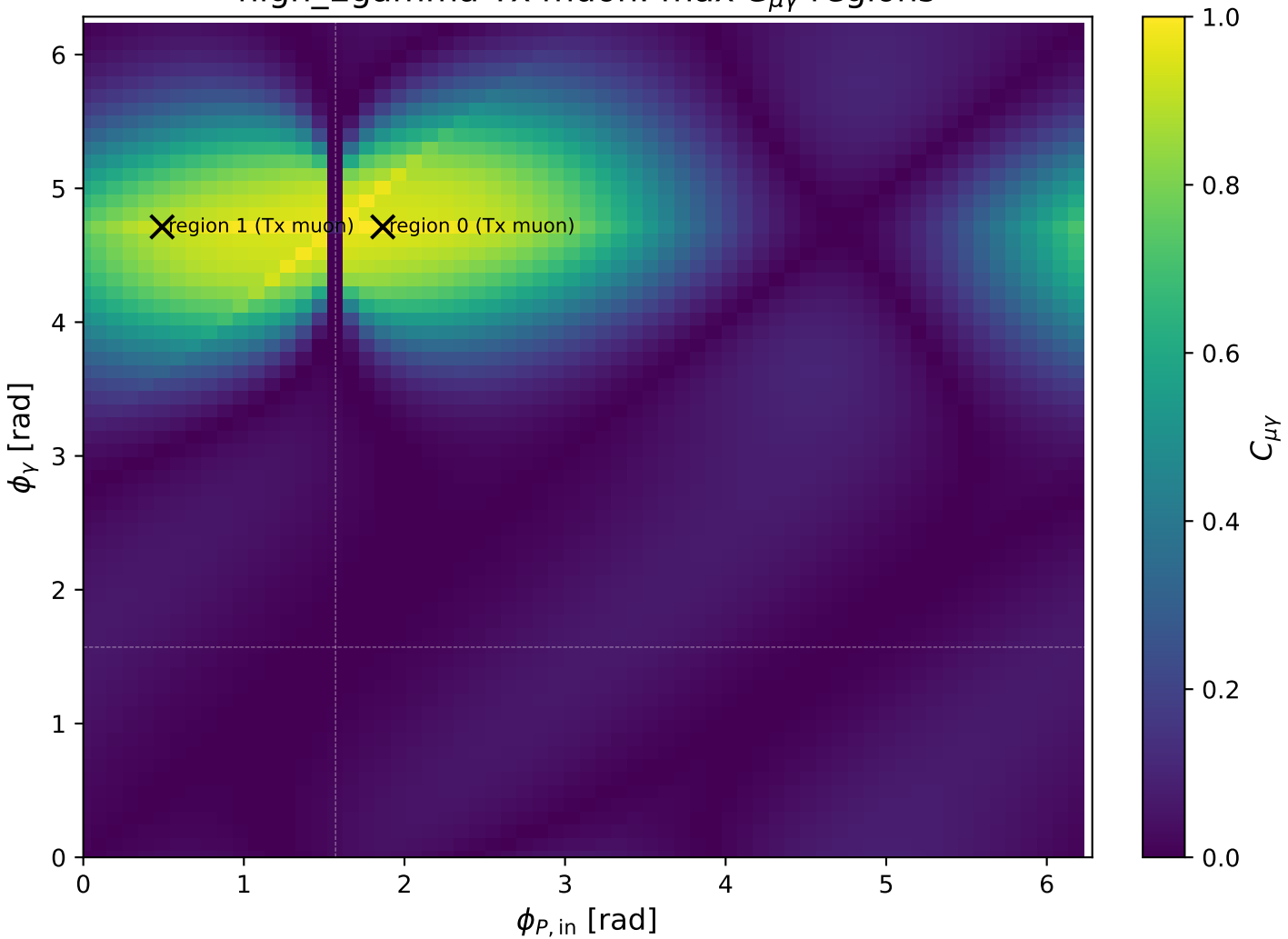
high_Egamma Tx muon: max C_{\mu\gamma} regions
