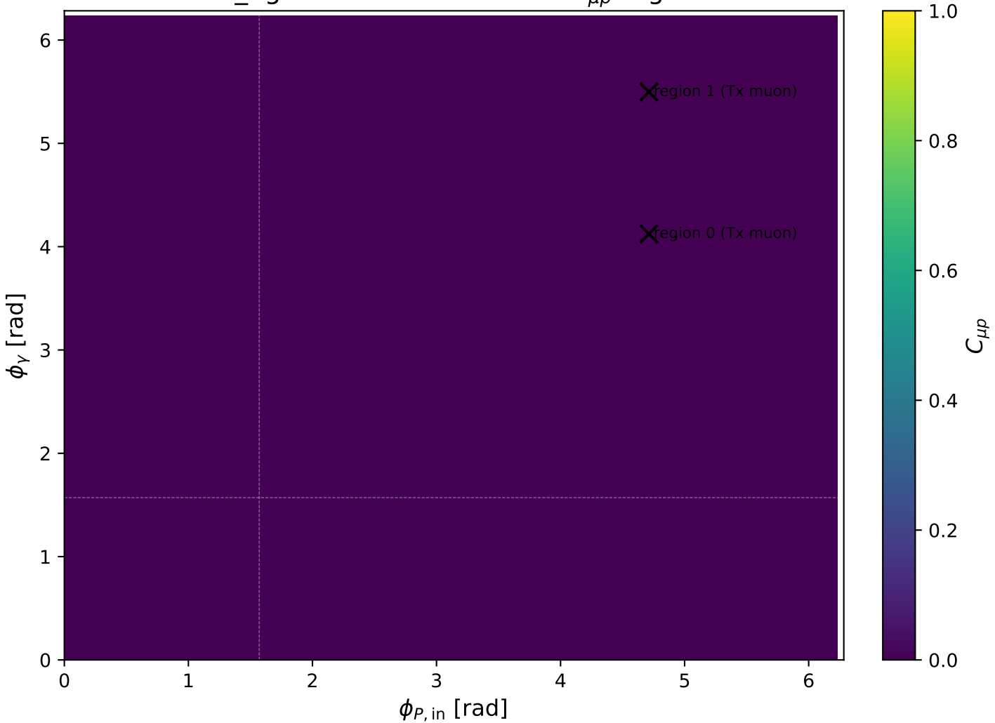
low_Egamma Tx muon: max C_{\mu p} regions
