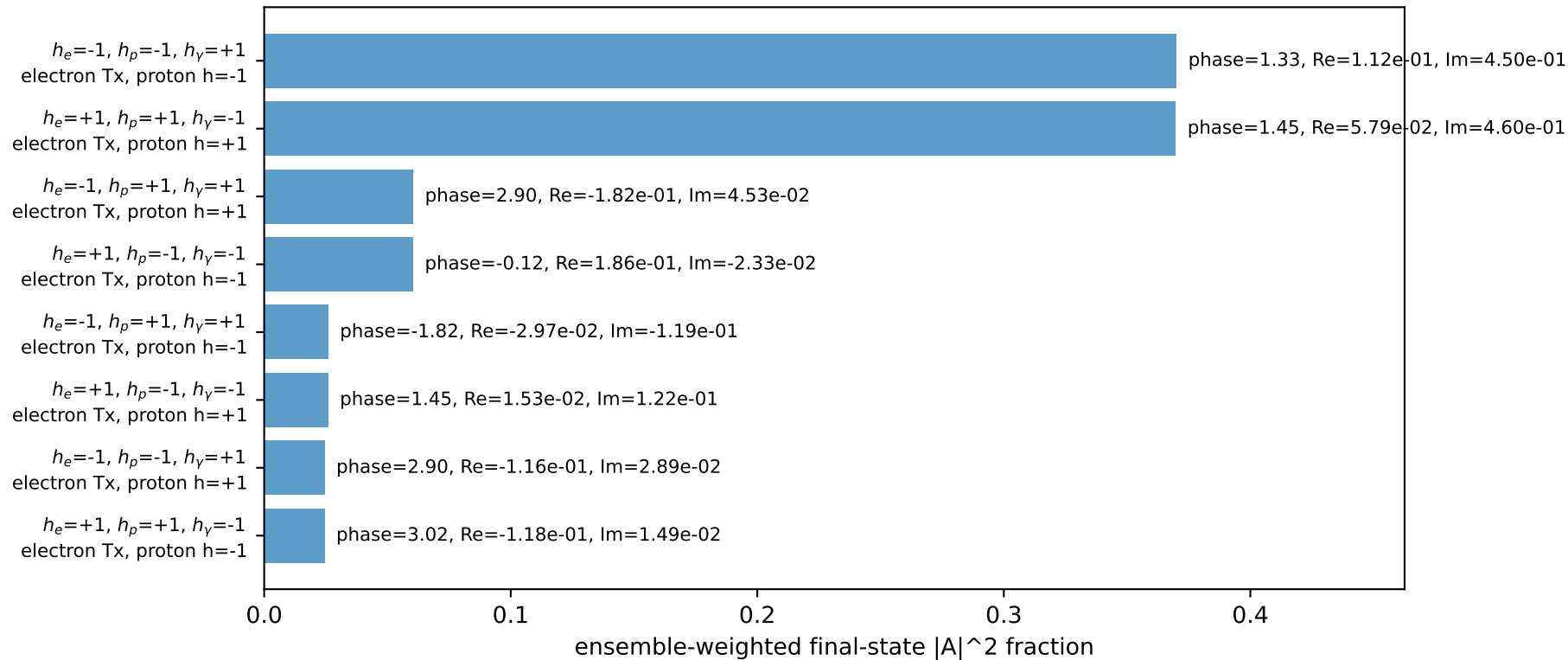
Leading initial-ensemble/final-state components (N=8, retained=96.1%)
