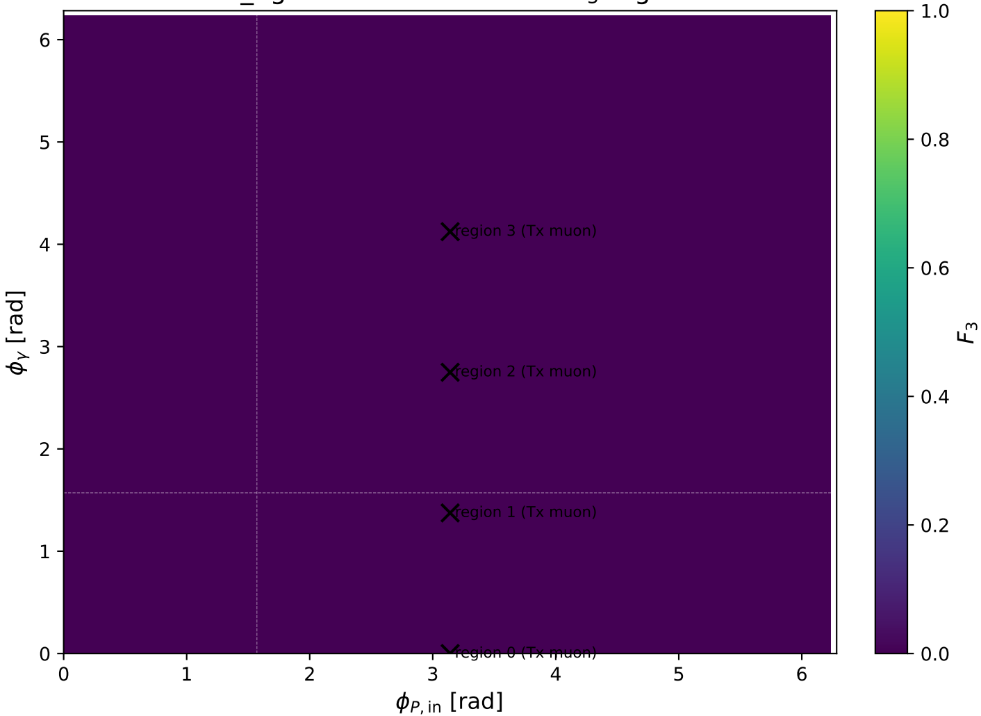
low_Egamma Tx muon: max F_3 regions
