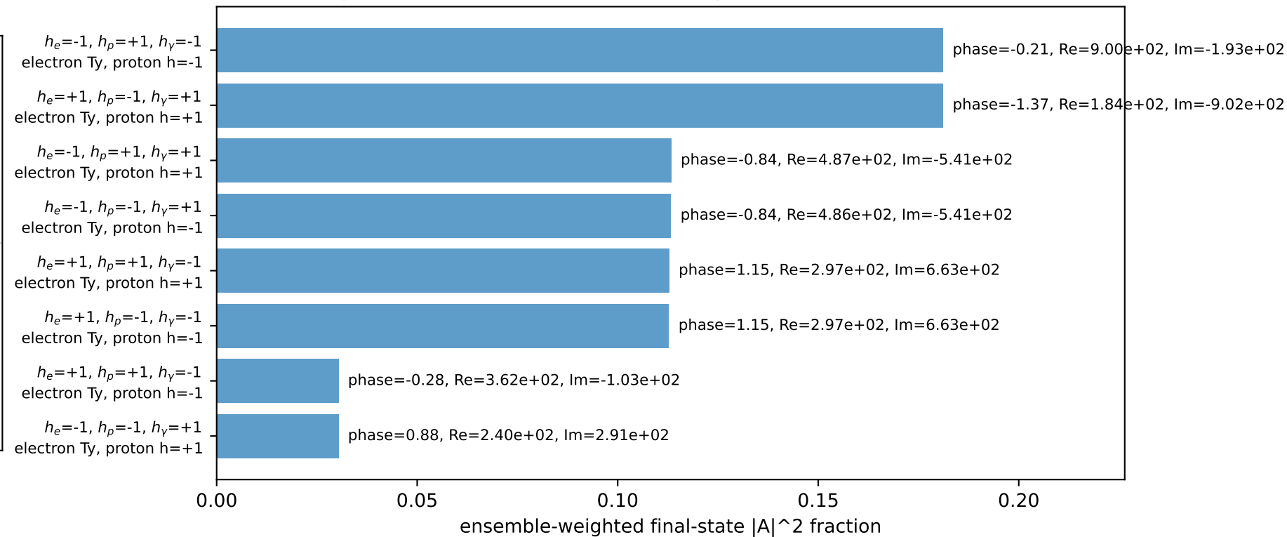
Leading initial-ensemble/final-state components (N=8, retained=87.5%)
