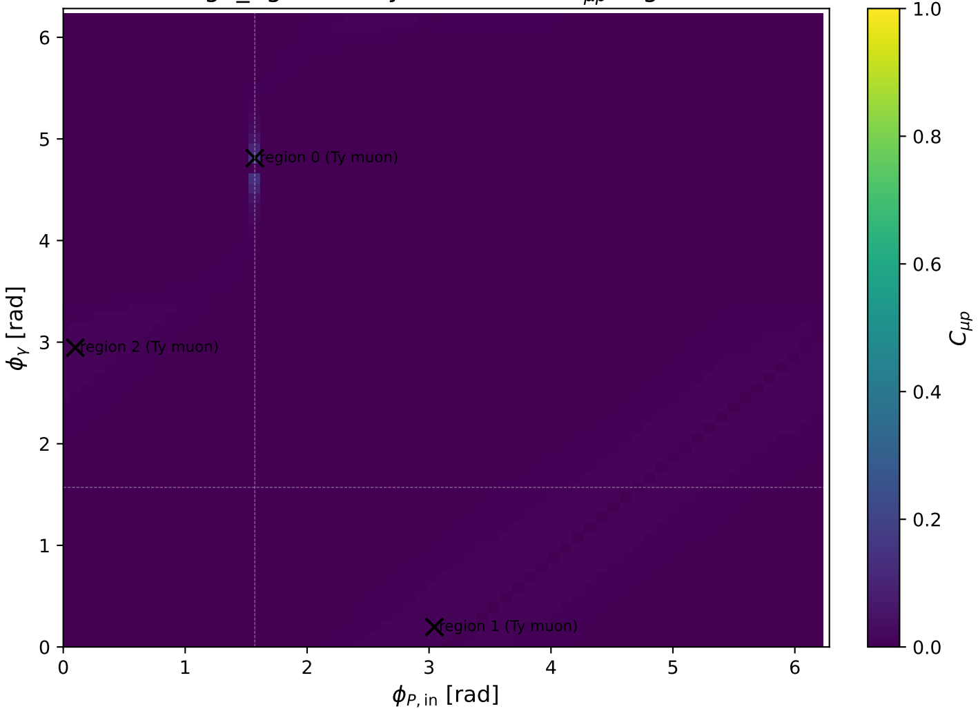
high_Egamma Ty muon: max C_{\mu p} regions
