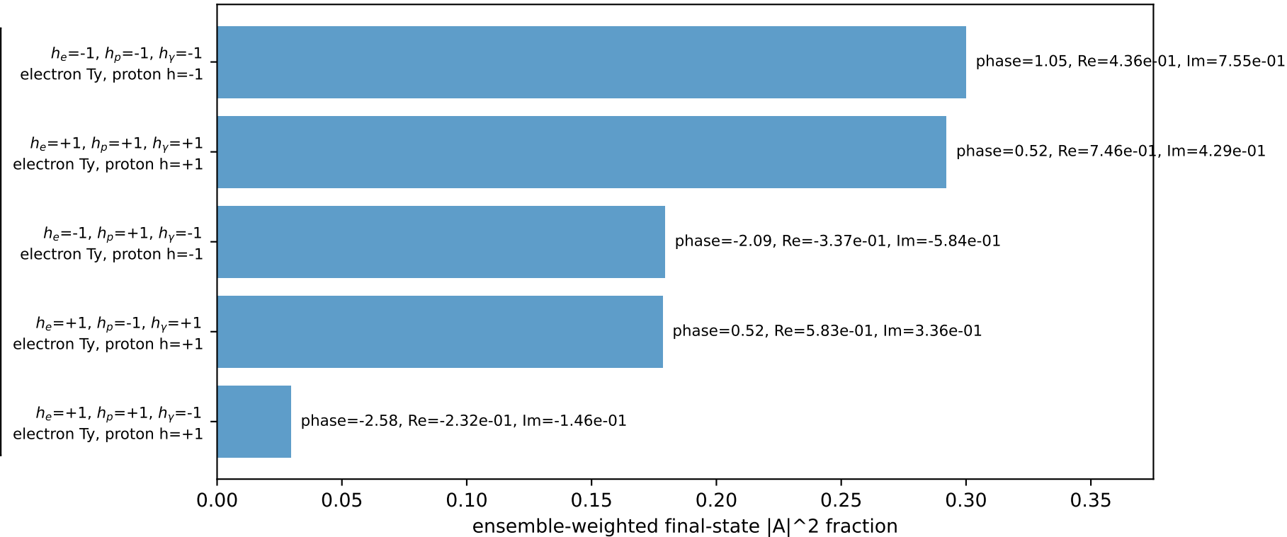
Leading initial-ensemble/final-state components (N=5, retained=98.0%)
