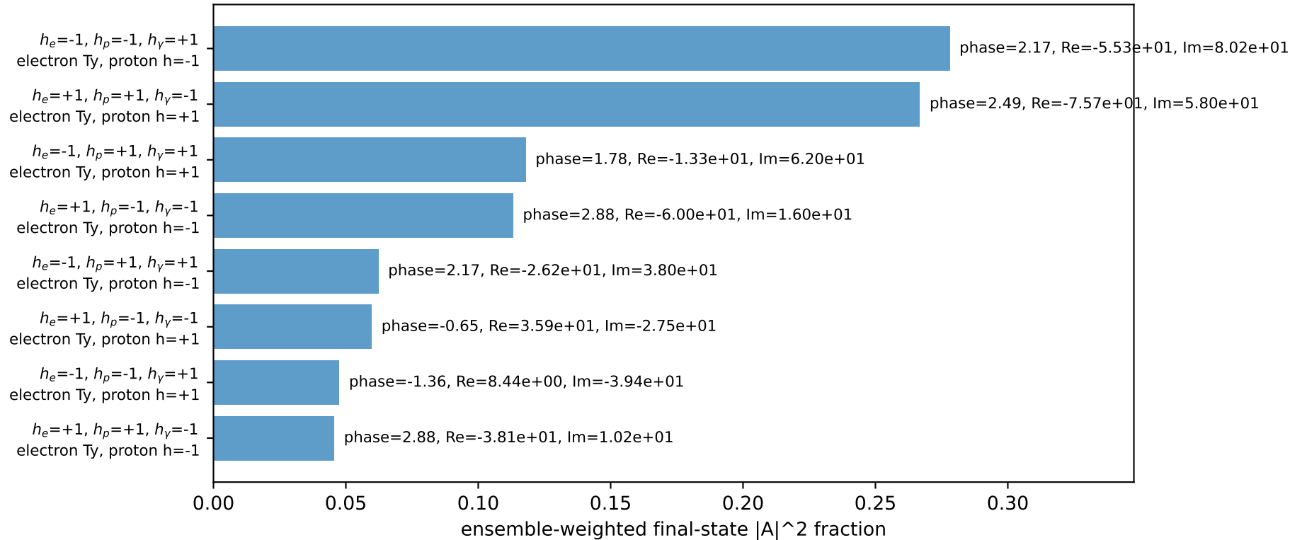
Leading initial-ensemble/final-state components (N=8, retained=99.1%)
