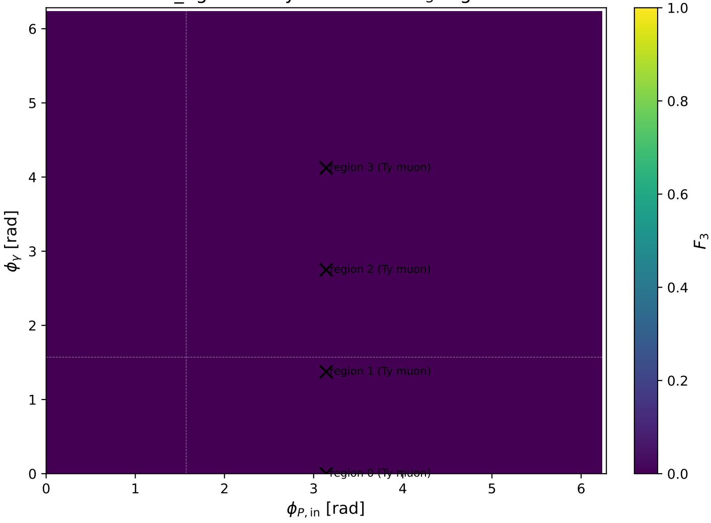
low_Egamma Ty muon: max F_3 regions
