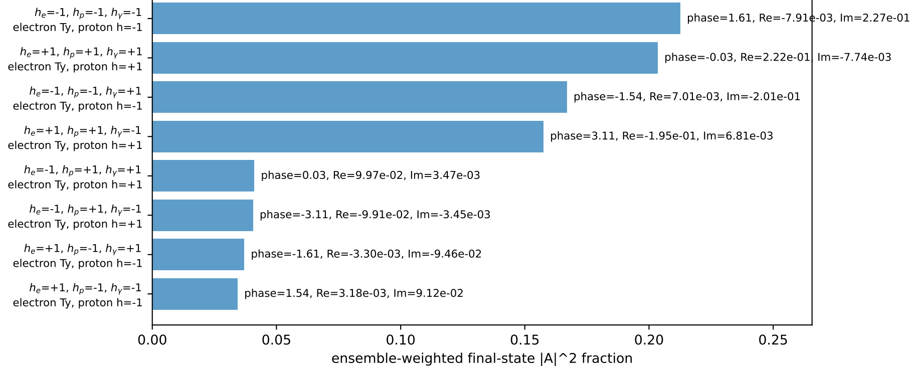
Leading initial-ensemble/final-state components (N=8, retained=89.3%)
