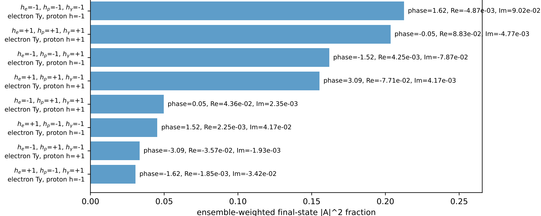
Leading initial-ensemble/final-state components (N=8, retained=89.2%)
