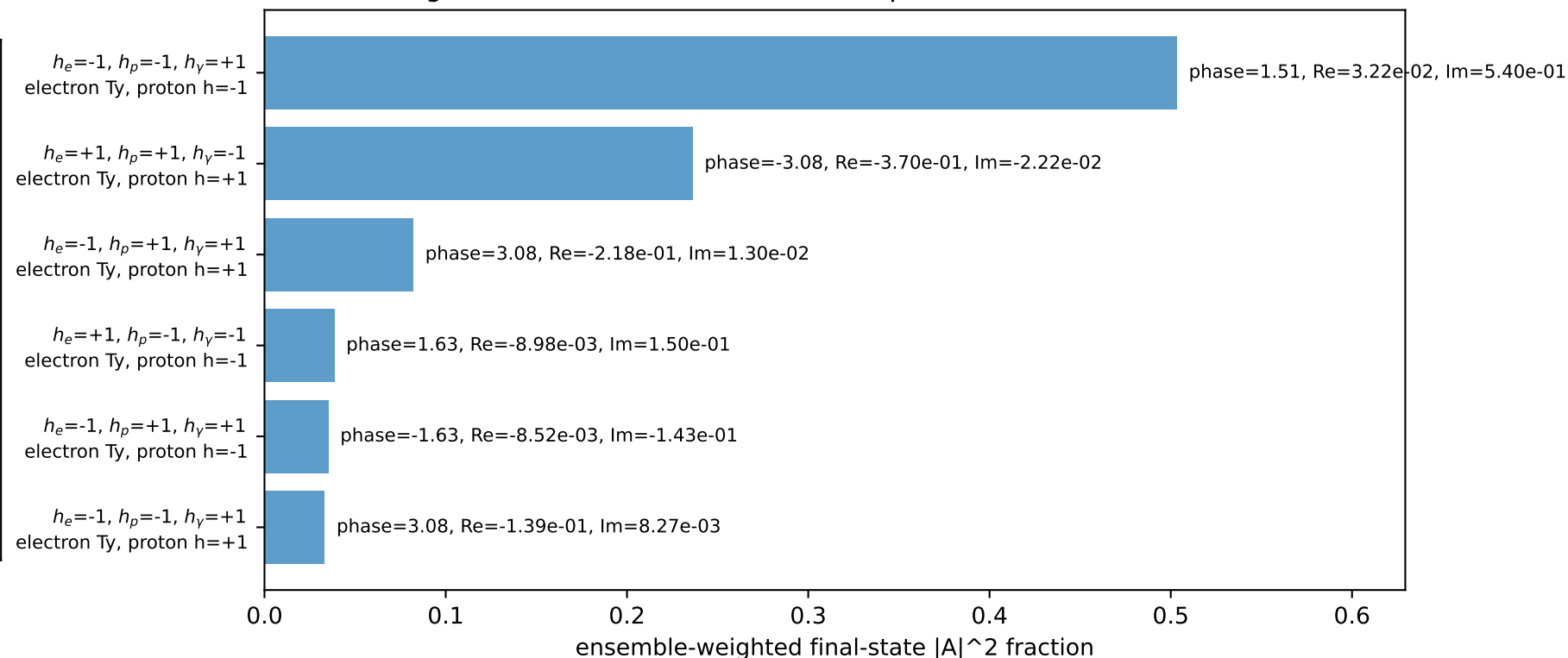
Leading initial-ensemble/final-state components (N=6, retained=92.9%)
