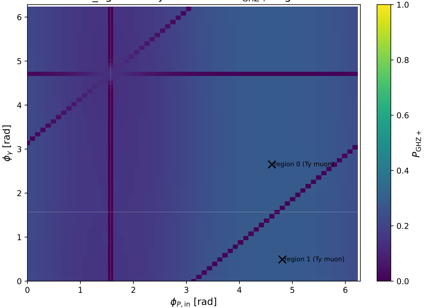
low_Egamma Ty muon: max P_{\text{GHZ}+} regions
